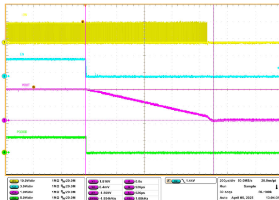
Figure 8-15. ENABLE Shutdown, 800kHz, FCCM, 15A Load, Soft-Off
