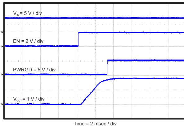
Figure 8-7. Power Up Relative To EN
