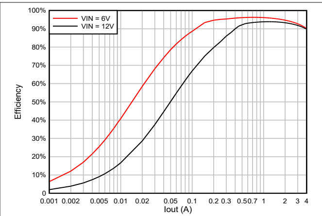
Figure 5-26. TPS564257C Efficiency at 3.3\text{V}_{\text{OUT}} With a 2.2\mu\text{H} Inductor
