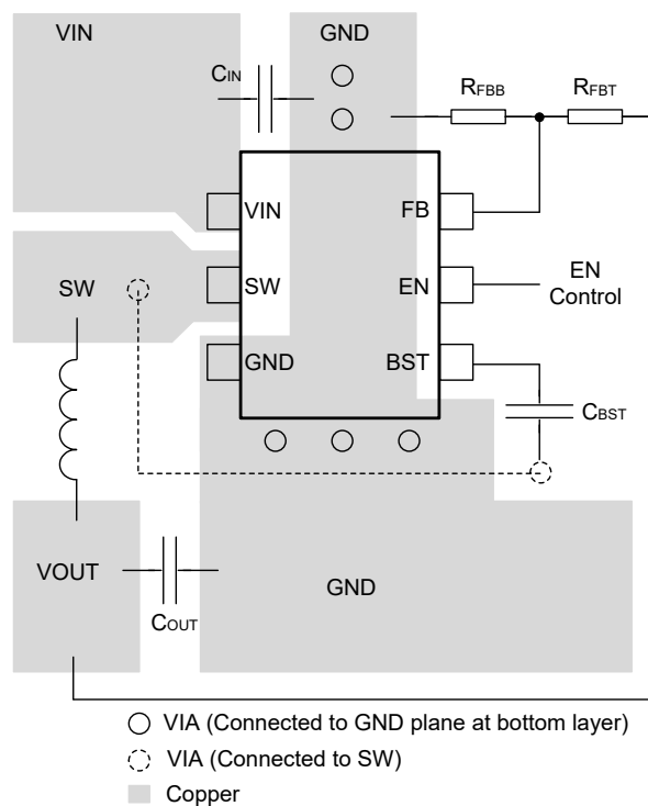
Figure 7-26. Suggested Layout
