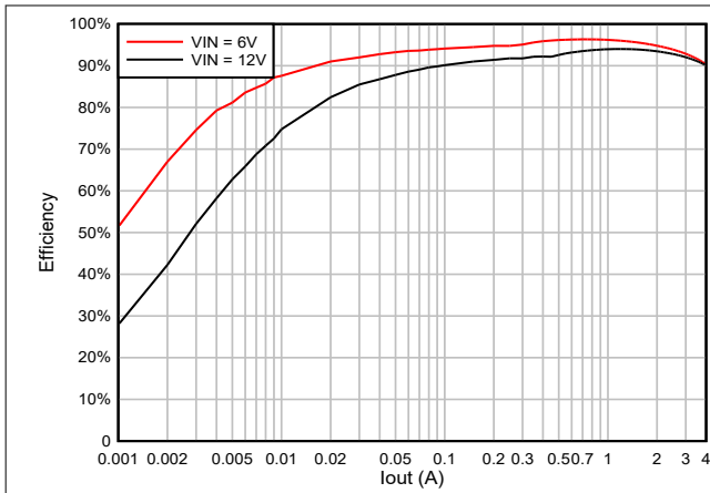
Figure 5-25. TPS564252C Efficiency at 3.3\text{V}_{\text{OUT}} With a 2.2\mu\text{H} Inductor
