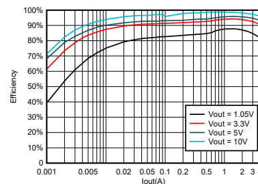
TPS564252B Efficiency at V_{IN} = 12\text{V}
