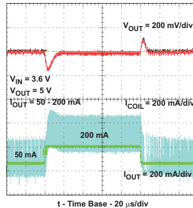
Figure 13. Load Transient Response 0 mA to 200 mA and 200 mA to 0 mA
