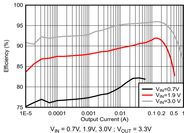
Figure 6-3. 3.3V VOUT Efficiency with Different Inputs Under Normal Mode
