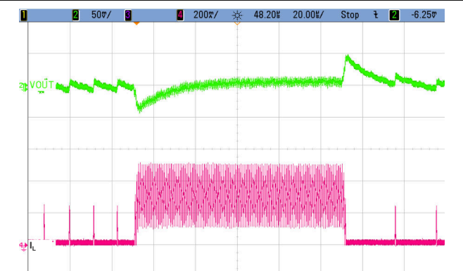
Figure 9-19. Load Transient Response; 5 mA to 290 mA
