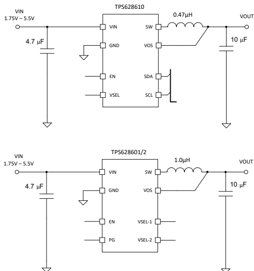
Typical Application
