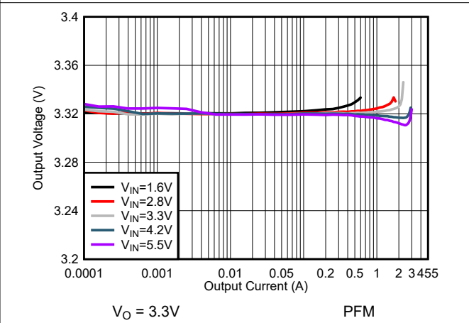
Figure 9-5. Load Regulation (PFM)
