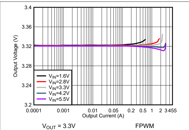
Figure 9-3. Load Regulation (FPWM)
