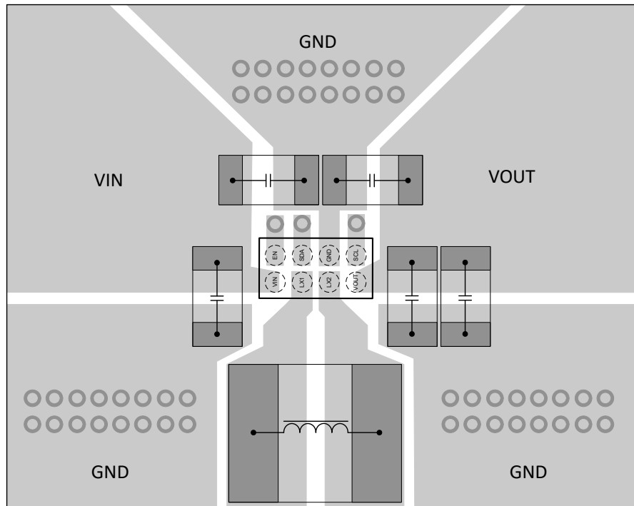
Figure 9-24. Layout Example
