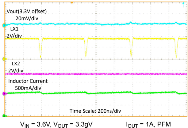
Figure 9-9. Switching Waveforms, Buck Operation with 1A Load
