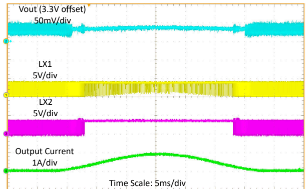
V_{IN} = 3.6V, V_{OUT} = 3.3V I_{OUT} = 100mA to 1A sweep
