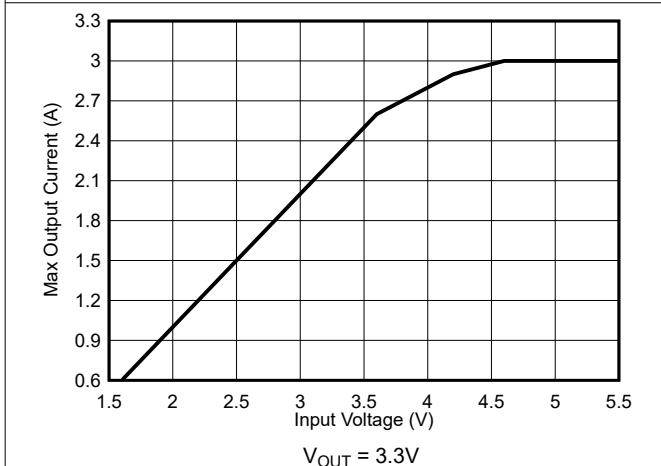
Figure 9-6. Typical Output Current Capability vs Input Voltage
