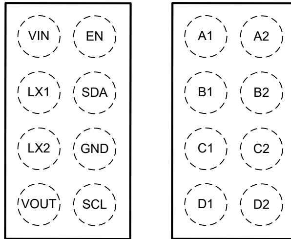
Figure 5-1. TPS631013A YBG Package, 8-Pin WCSP (Top View)
