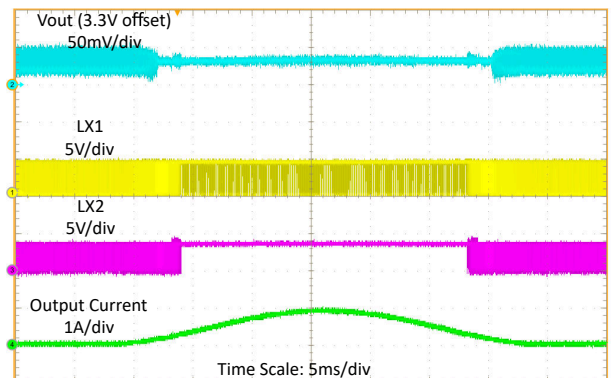
V_{IN} = 4.3V, V_{OUT} = 3.3V I_{OUT} = 100mA to 1A sweep
