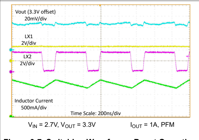
Figure 9-7. Switching Waveforms, Boost Operation with 1A Load
