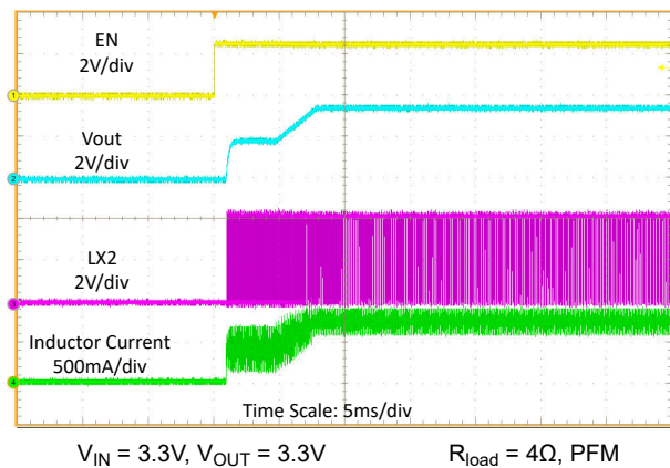
Figure 9-12. Start-Up by EN (Measured on TPS631013A)
