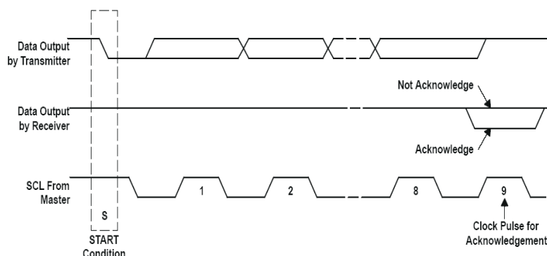
Figure 9-4. Acknowledge on the I 2 C Bus
