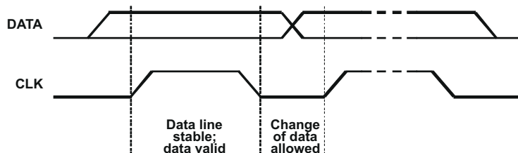
Figure 9-3. Bit Transfer on the Serial Interface
