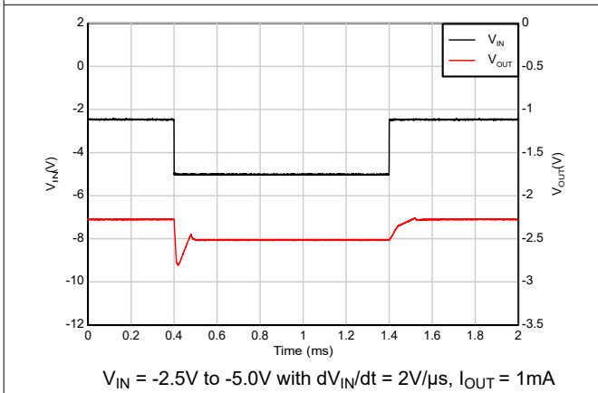
Figure 5-41. TPS72325 Dropout exit Response (new chip)
