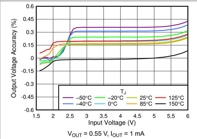
Figure 5-2. 0.55-V Line Regulation vs V_{IN}
