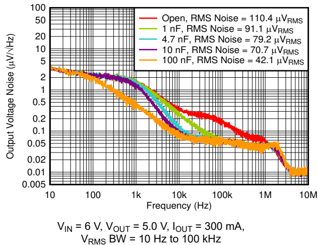
Figure 6-31. Output Noise vs Frequency and C_{FF}
