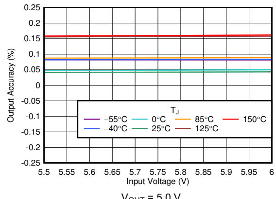
Figure 6-6. Output Accuracy vs V_{\text{IN}}
