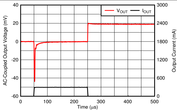
V_{\text{OUT}} = 1.2\text{ V} , I_{\text{OUT}} = 0\text{ mA to }300\text{ mA} , I_{\text{OUT}} slew rate = 1\text{ A}/\mu\text{s} , T_J = -40^\circ\text{C}
