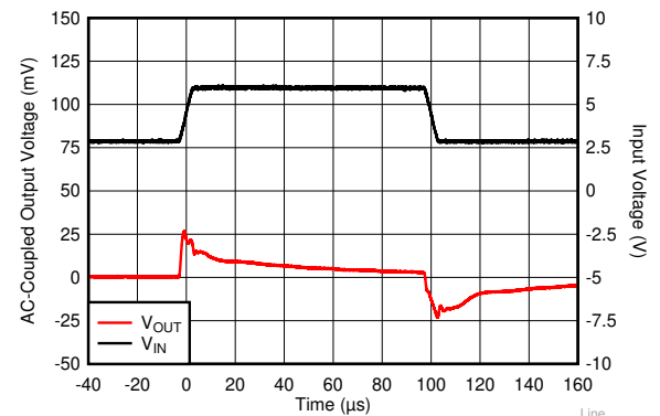
Figure 6-24. V_{IN} Transient From 2.8 V to 6.0 V
