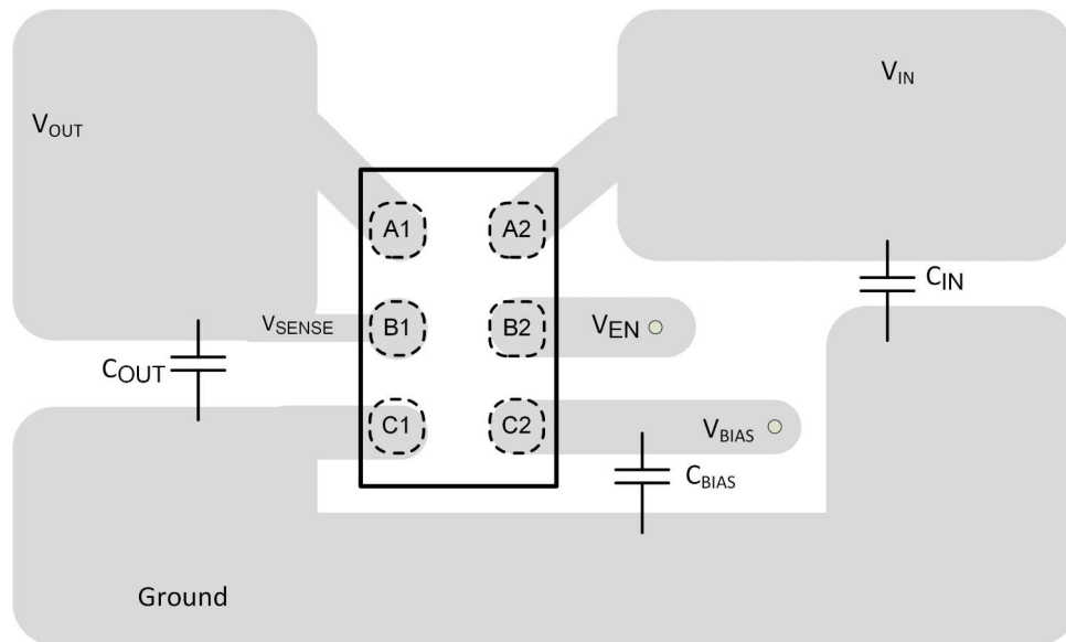
Figure 7-6. Recommended Layout (YCK Package)
