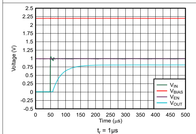
Figure 5-11. Start-Up With V_{\text{BIAS}} and V_{\text{EN}} Before V_{\text{IN}}
