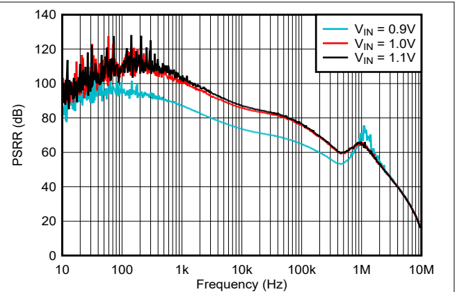
Figure 5-14. V_{IN} PSRR vs Frequency and V_{IN}
