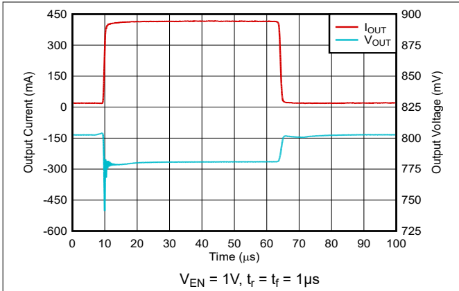
Figure 5-13. Load Transient From 100µA to 400mA
