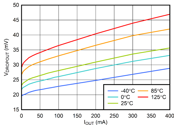
Figure 7-5. V IN Dropout Voltage vs I OUT
