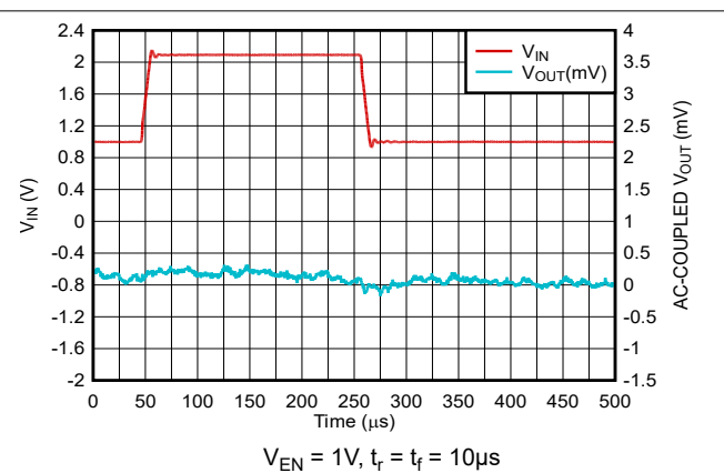
Figure 5-12. Line Transient From 1V to 2.2V
