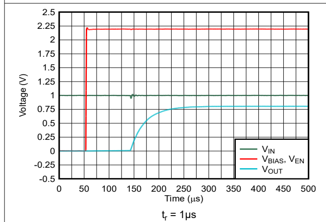
Figure 5-9. Start-Up With V_{\text{IN}} Before V_{\text{BIAS}} and V_{\text{EN}}
