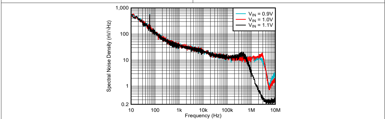
Figure 5-17. Output Noise vs Frequency and I_{OUT}
