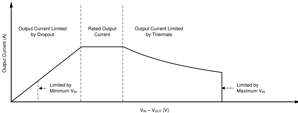
Figure 7-3. Continuous Operation Diagram With Description of Regions
