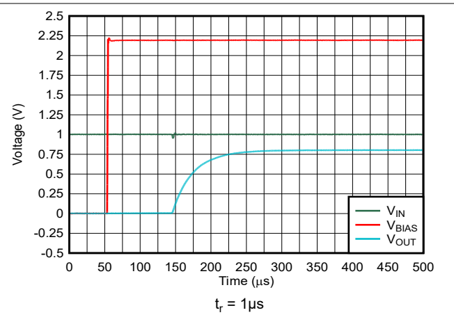
Figure 5-8. Start-Up With V_{\text{IN}} and Enable Before V_{\text{BIAS}}
