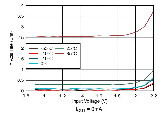
Figure 5-7. V_{\text{IN}} Input Current vs V_{\text{IN}} in Shutdown
