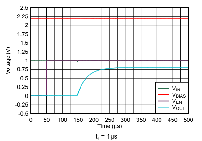
Figure 5-10. Start-Up With V_{\text{IN}} and V_{\text{BIAS}} Before V_{\text{EN}}
