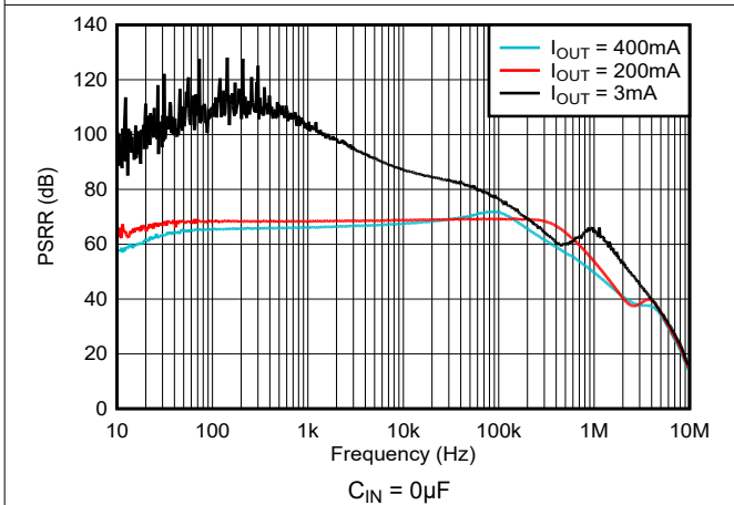
Figure 5-15. V_{IN} PSRR vs Frequency and I_{OUT}
