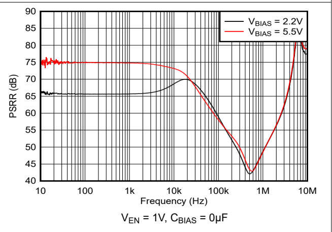
Figure 5-16. V_{BIAS} PSRR vs Frequency and V_{BIAS} - V_{OUT}
