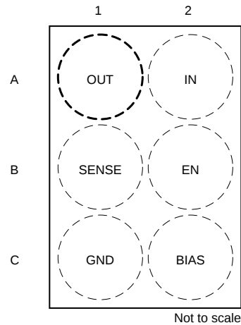
Figure 4-1. YCK Package, 6-Pin WCSP, 0.35mm Pitch (Top View)
