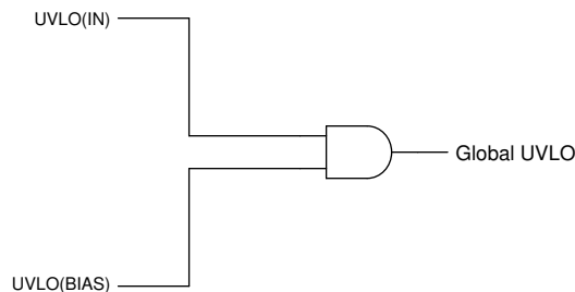
Figure 6-1. Global UVLO Circuit
