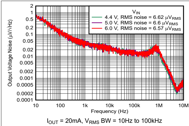
Figure 5-31. Noise vs Frequency and V_{IN}
