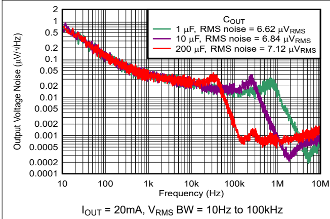
Figure 5-33. Noise vs Frequency and C_{OUT}
