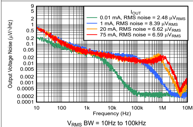
Figure 5-35. Noise vs Frequency and I_{OUT}
