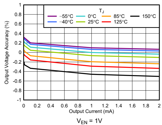
Figure 5-4. Output Voltage Accuracy vs I_{OUT}
