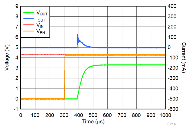
Figure 6-24. Start-Up Inrush Current
