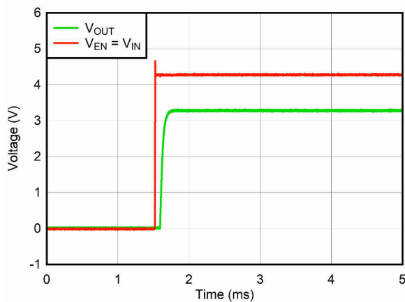
Figure 6-23. Start-Up With V_{EN} = V_{IN}
