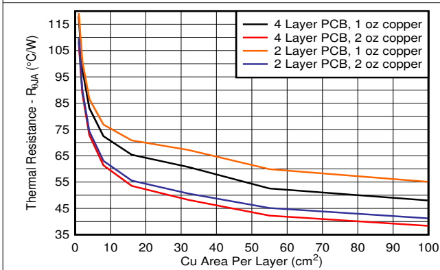
Figure 7-4. R_{\theta JA} vs Copper Area 2s2p DCY Package
