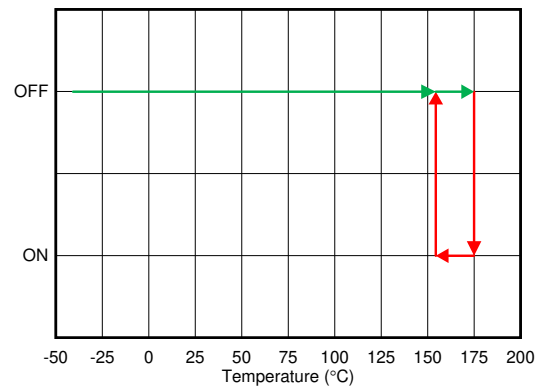
Figure 5-32. Thermal Shutdown
