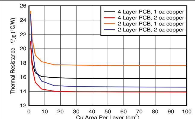
Figure 7-3. \psi_{JB} vs Copper Area 2s2p DRB Package
