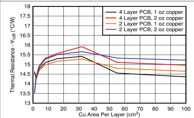
Figure 7-5. \psi_{JB} vs Copper Area 2s2p DCY Package
