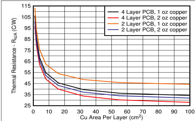
Figure 7-2. R_{\theta JA} vs Copper Area 2s2p DRB Package
