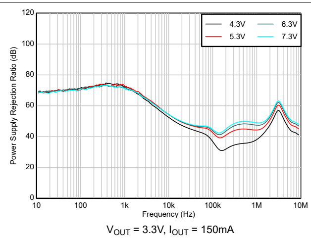
Figure 5-20. Ripple Rejection vs Frequency, Input Voltage
