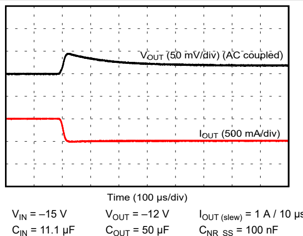
Figure 6-24. Load Step: 1 mA to 500 mA
