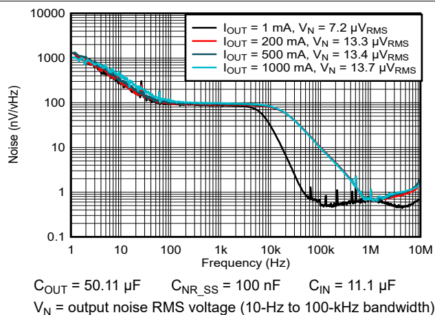
Figure 6-20. Output Noise vs Frequency Across Output Current (Noise Spectral Density)
