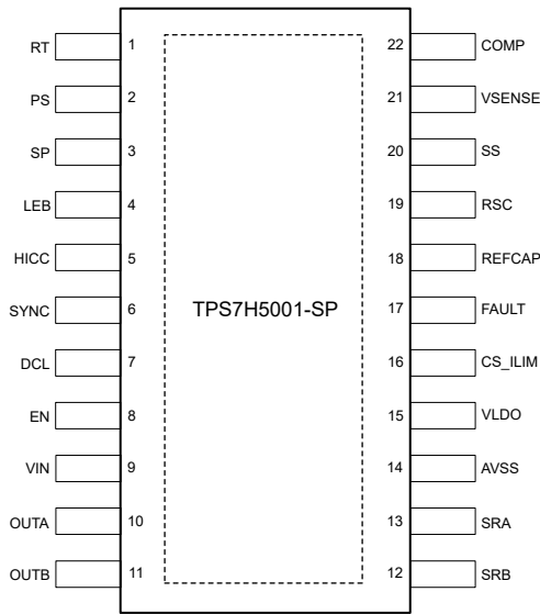
Figure 6-1. TPS7H5001-SP HFT Package 22-Pin CFP With Thermal Pad (Top View)
