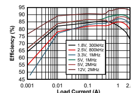
Efficiency vs Output Current V_{IN} = 24\text{V}
