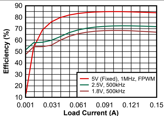
Figure 8-6. 12VIN Efficiency
