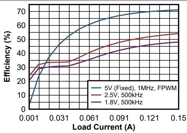
Figure 8-10. 48VIN Efficiency
