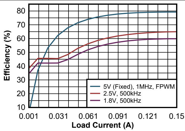
Figure 8-8. 24VIN Efficiency
