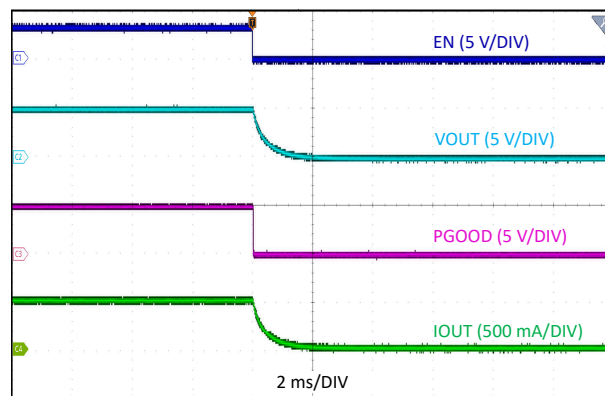
Figure 8-4. Shutdown Waveforms
