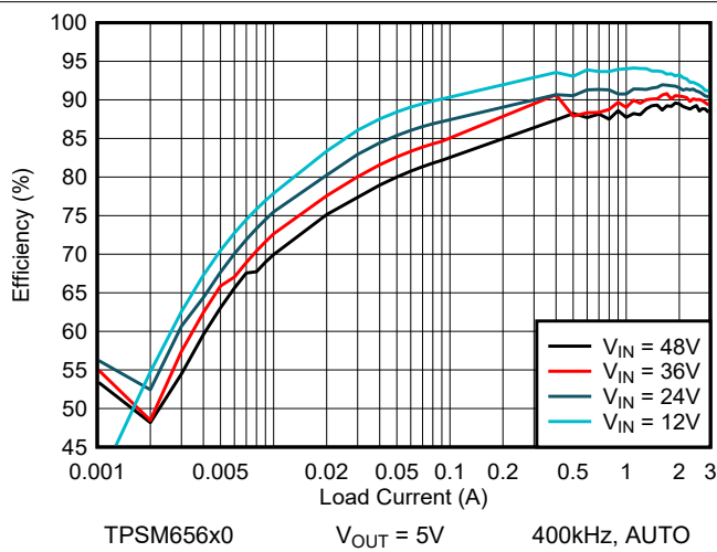
Figure 8-5. Efficiency
