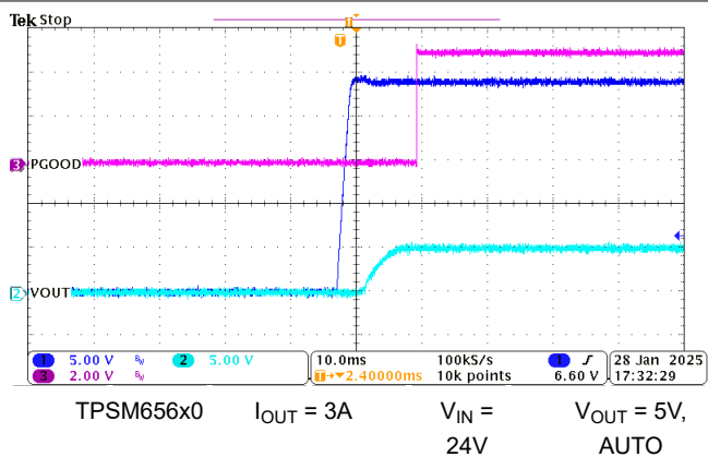
Figure 8-9. Start-Up
