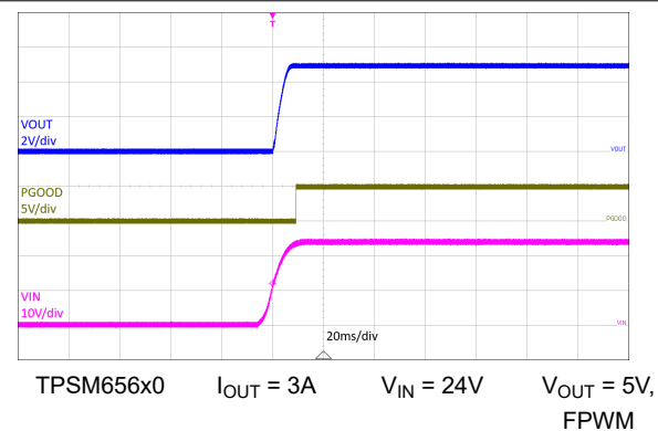
Figure 8-16. Start-Up
