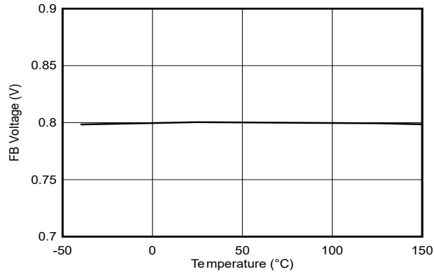
Figure 6-1. Feedback Voltage
