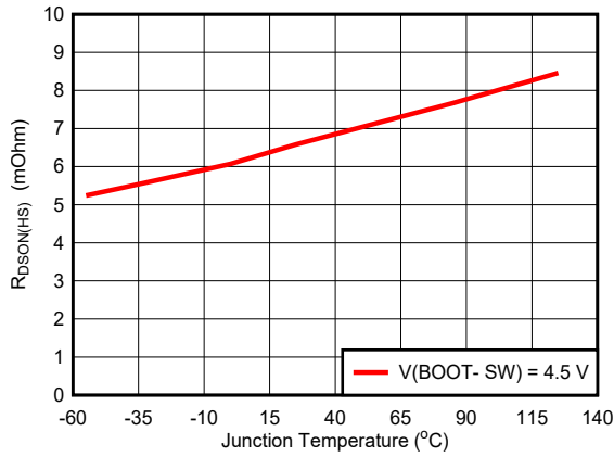
Figure 6-1. High-Side FET R_{dsON}
