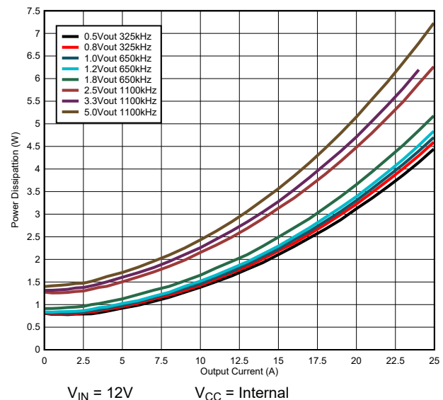
Figure 5-4. TPSM8S6B24S Power Dissipation vs Output Current
