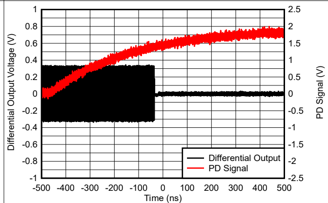
Figure 5-48. Step Response
