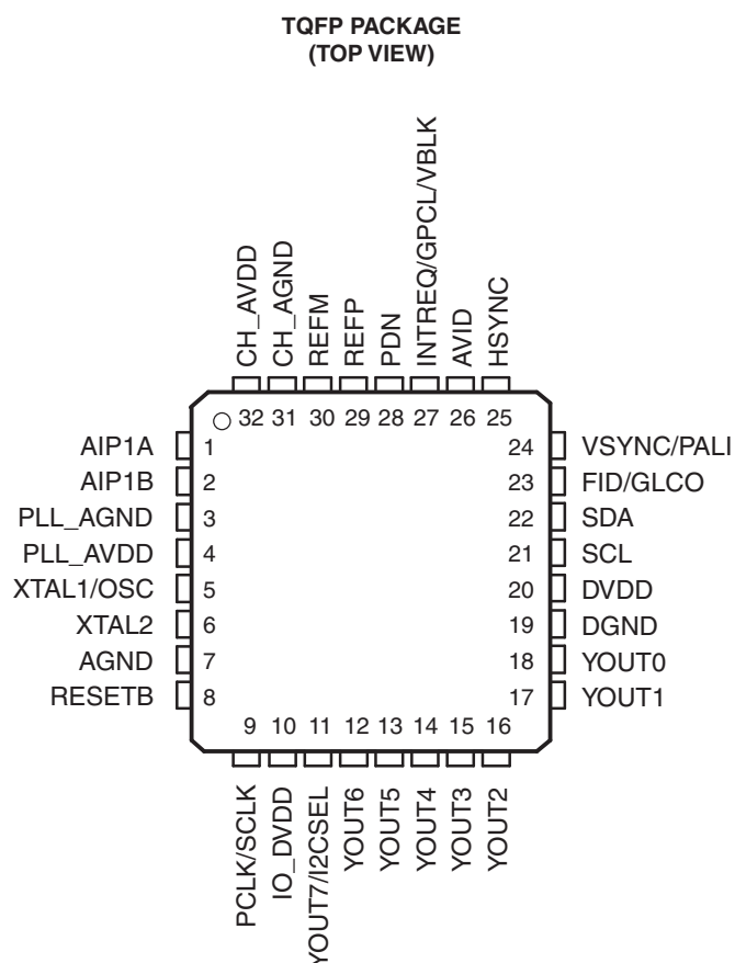
Figure 2-2. Terminal Diagrams
