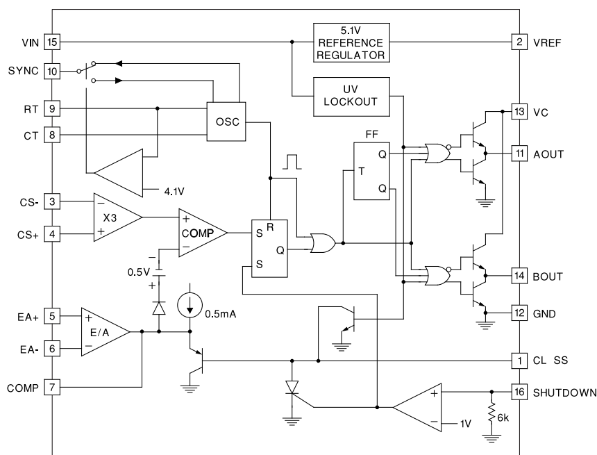
Block Diagram
