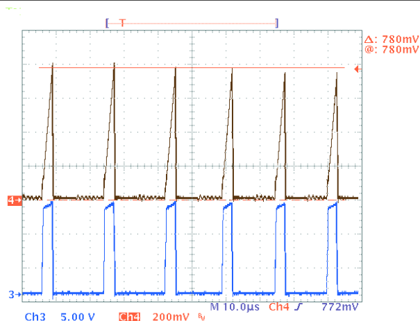
Figure 8-5. EMI Dithering
