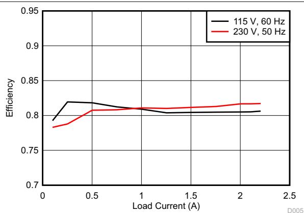
Figure 8-6. Efficiency
