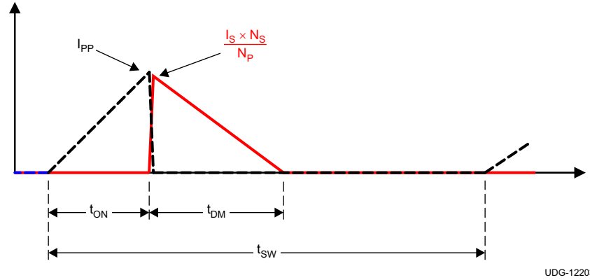
Figure 7-6. Transformer-Current Relationship
