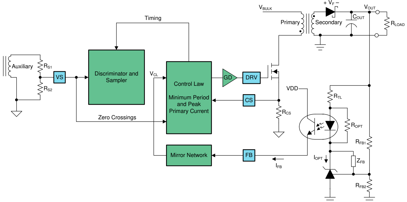
Figure 7-2. Simplified Flyback Convertor (With the Main Voltage Regulation Blocks)
