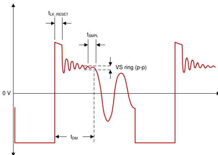
Figure 7-4. Auxiliary-Winding Waveform Details
