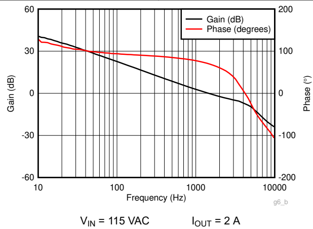
Figure 8-11. Bode Plot
