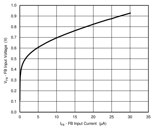
Figure 6-9. FB Input Voltage vs. FB Input Current
