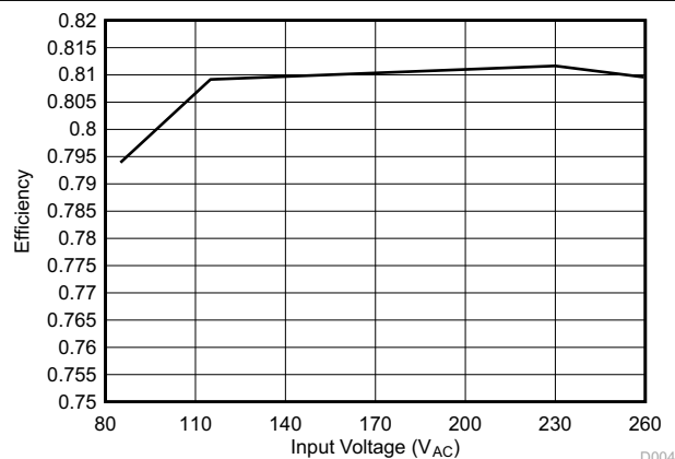
Figure 8-7. Average Efficiency
