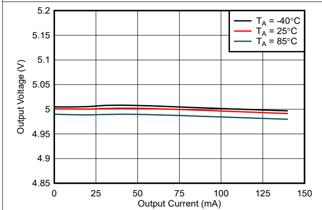
Figure 6-23. Output Voltage Regulation ( V_{VCC} ) vs Load Current ( I_{VCC} ): V_{CC} = 5.0V , V_{INP} = 3.3V , C_{OUT2} = 22\mu F
