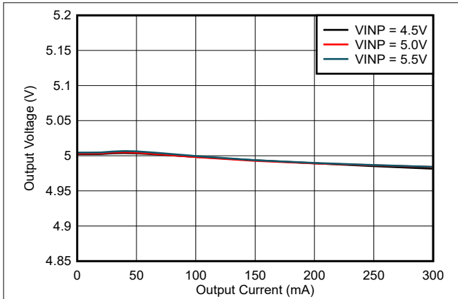
Figure 6-19. Output Voltage Regulation ( V_{VCC} ) vs Load Current ( I_{VCC} ): V_{CC} = 5.0V , T_A = 25^\circ C , C_{OUT2} = 22\mu F
