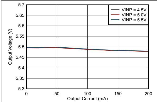
Figure 6-21. Output Voltage Regulation ( V_{VCC} ) vs Load Current ( I_{VCC} ): V_{CC} = 5.5V , T_A = 25^\circ C , C_{OUT2} = 22\mu F
