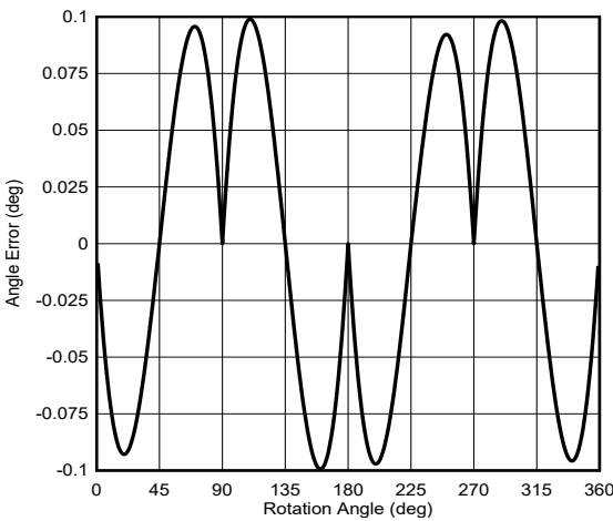
Figure 6-2. 8-point Linearization
