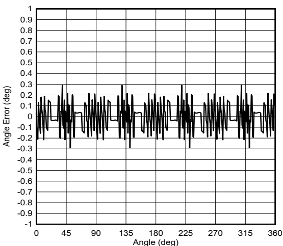
Figure 5-2. 8-bit Quantization Error
