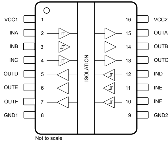
Figure 4-1. Pin Diagram (DW-16 Wide-SOIC Package)
