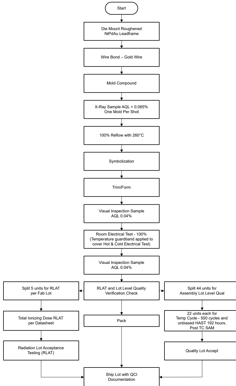
Figure 1-1. SN54SC1G08-SEP Space Enhanced Plastic Production Flow Chart
