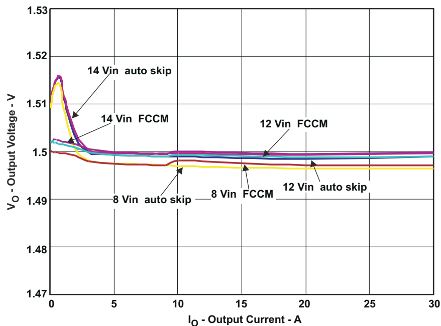
Figure 7-2. Load Regulation
