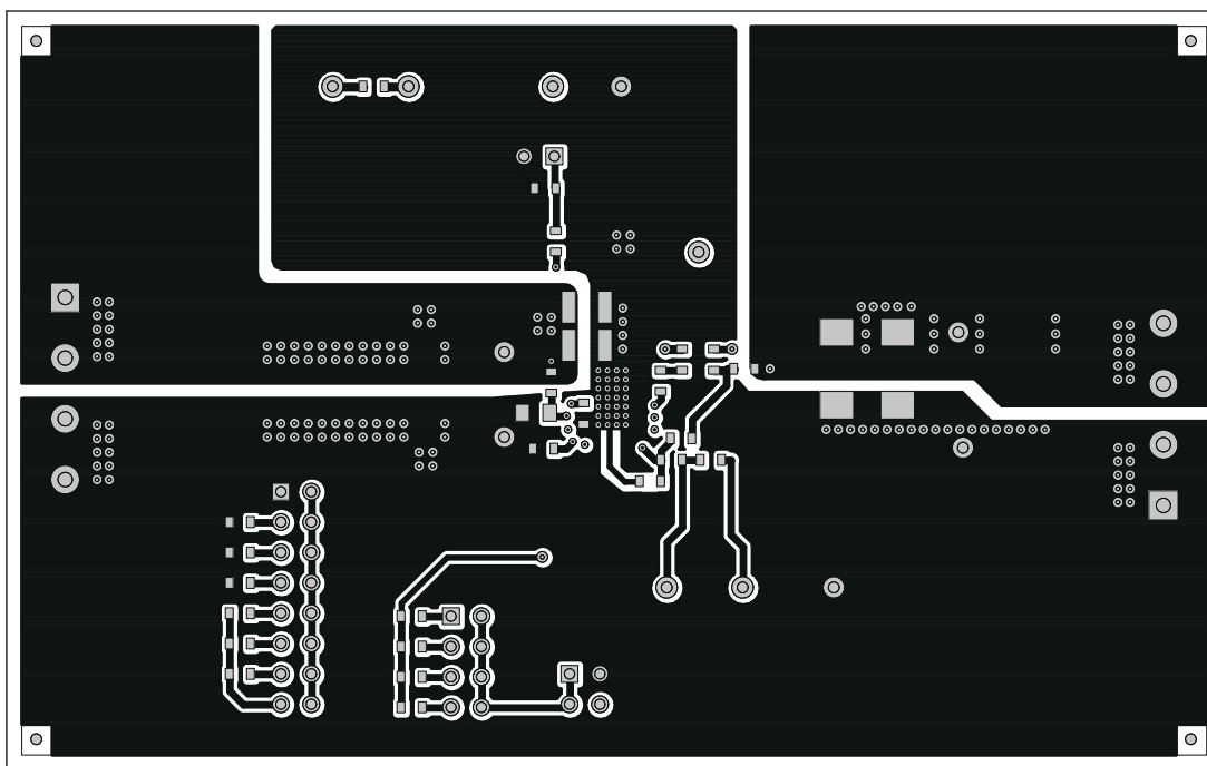
Figure 8-8. TPS53355EVM-743 Bottom Layer Copper
