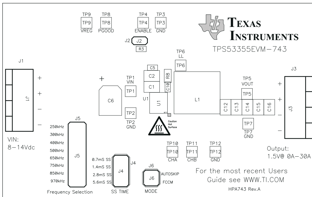
Figure 8-1. TPS53355EVM-743 Top Layer Assembly Drawing
