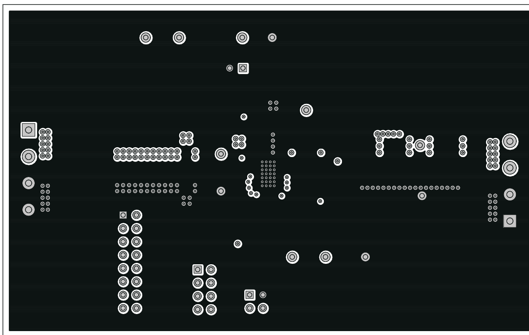
Figure 8-7. TPS53355EVM-743 Layer-5 Copper
