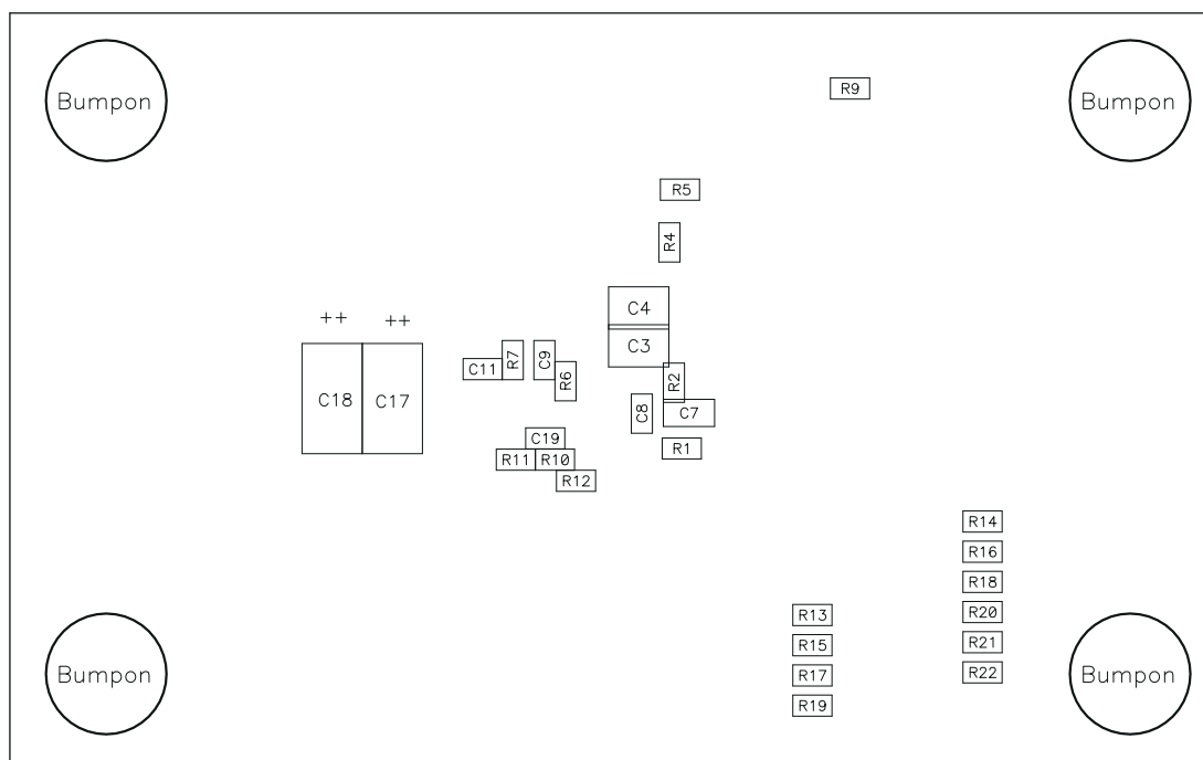
Figure 8-2. TPS53355EVM-743 Bottom Assembly Drawing
