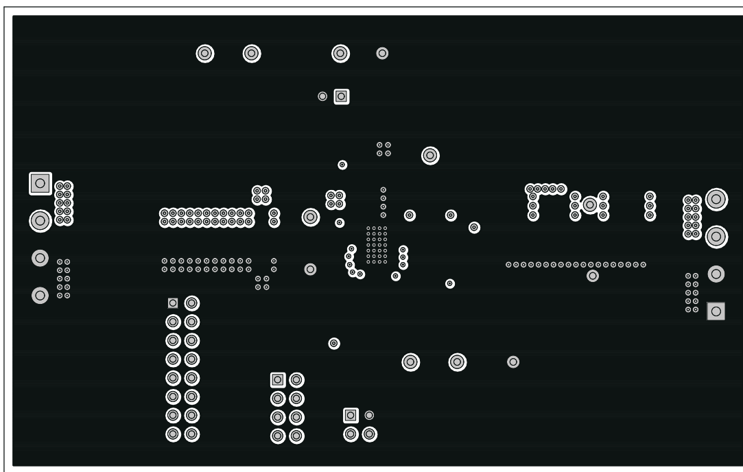
Figure 8-4. TPS53355EVM-743 Layer-2 Copper
