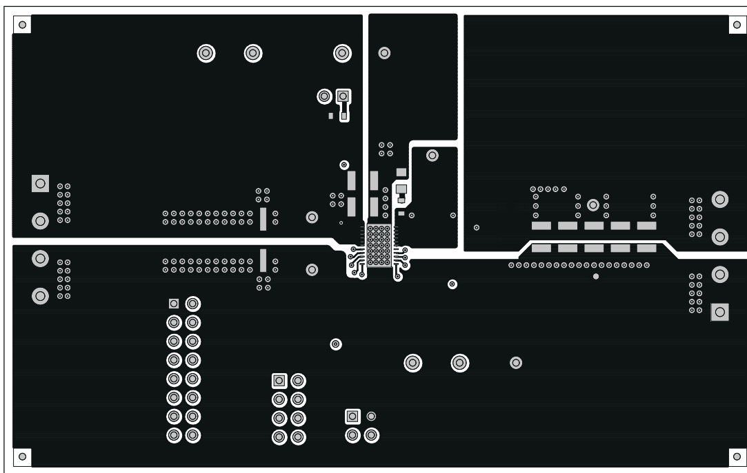
Figure 8-3. TPS53355EVM-743 Top Copper
