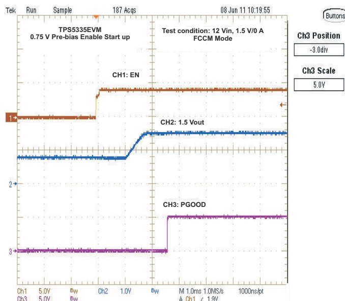
Figure 7-11. Output 0.75-V Prebias Turn-On
