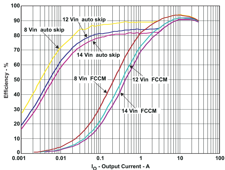
Figure 7-1. Efficiency
