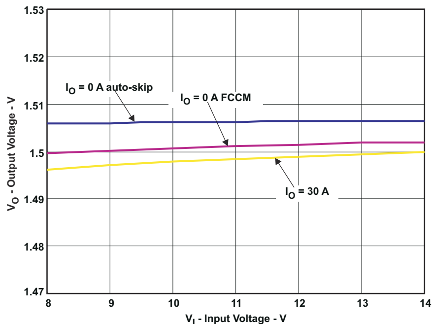
Figure 7-3. Line Regulation
