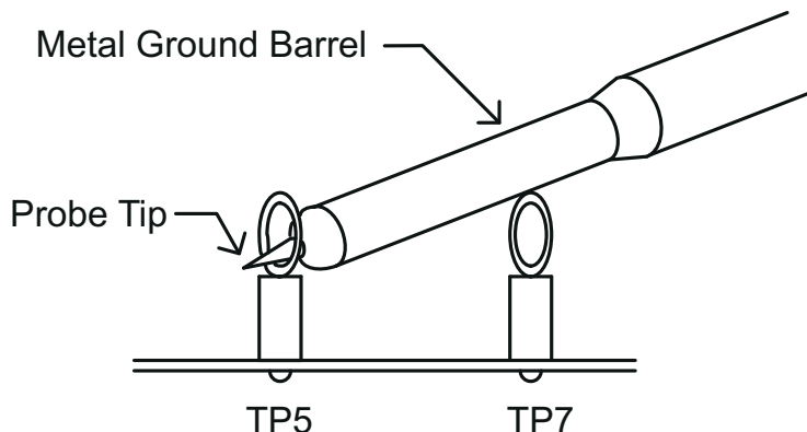
Figure 4-1. Tip and Barrel Measurement for VOUT Ripple
