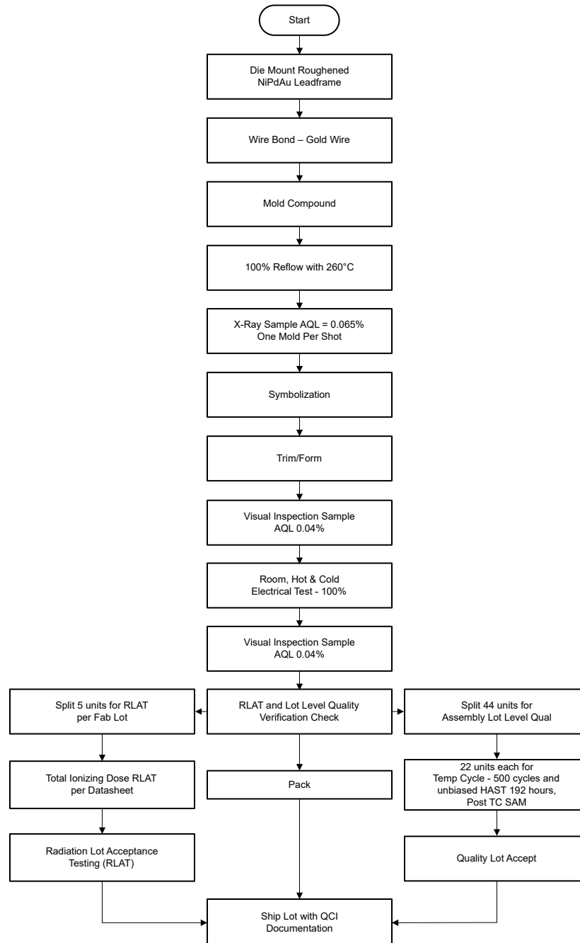
Figure 1-1. OPA4H838-SEP Space Enhanced Plastic Production Flow Chart
