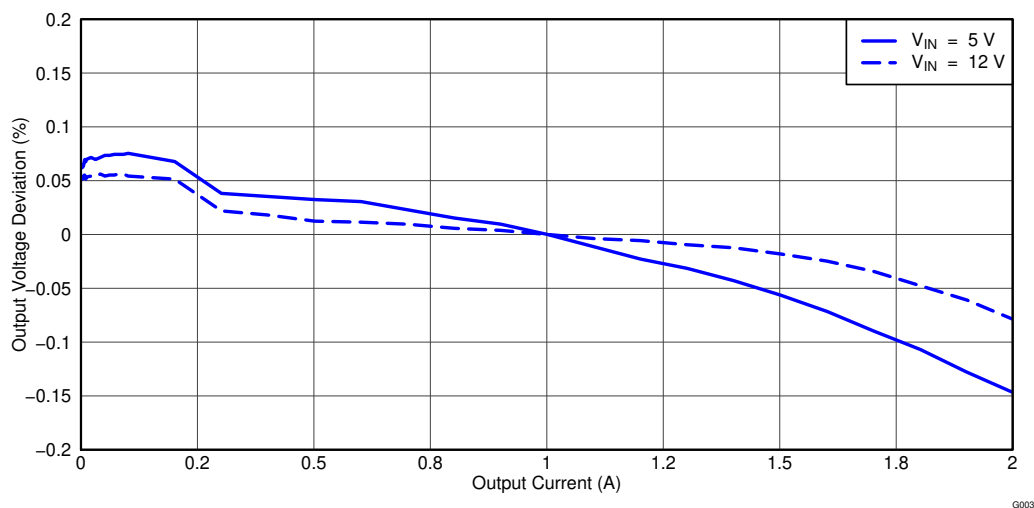
Figure 4-3. TPS54229EVM-056 Load Regulation, V_{IN} = 5\text{ V} and V_{IN} = 12\text{ V} .
