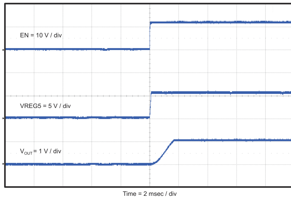
Figure 4-11. TPS54229EVM-056 Start-Up Relative to EN With VREG5
