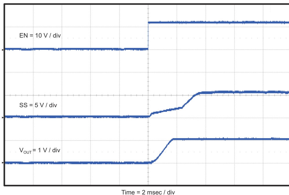
Figure 4-10. TPS54229EVM-056 Start-Up Relative to EN With SS
