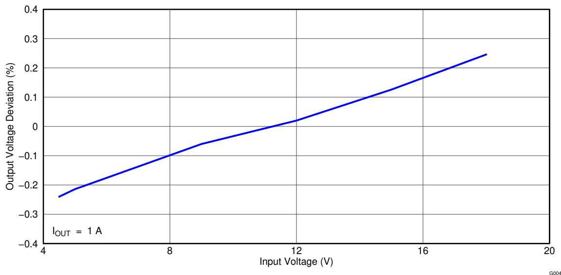
Figure 4-4. TPS54229EVM-056 Line Regulation
