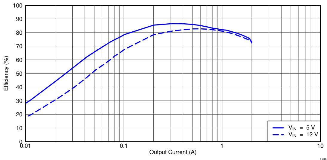
Figure 4-2. TPS54229EVM-056 Light-Load Efficiency
