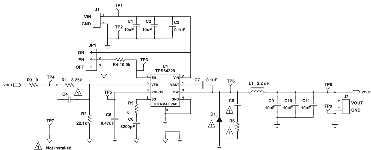
Figure 6-1. TPS54229EVM-056 Schematic Diagram
