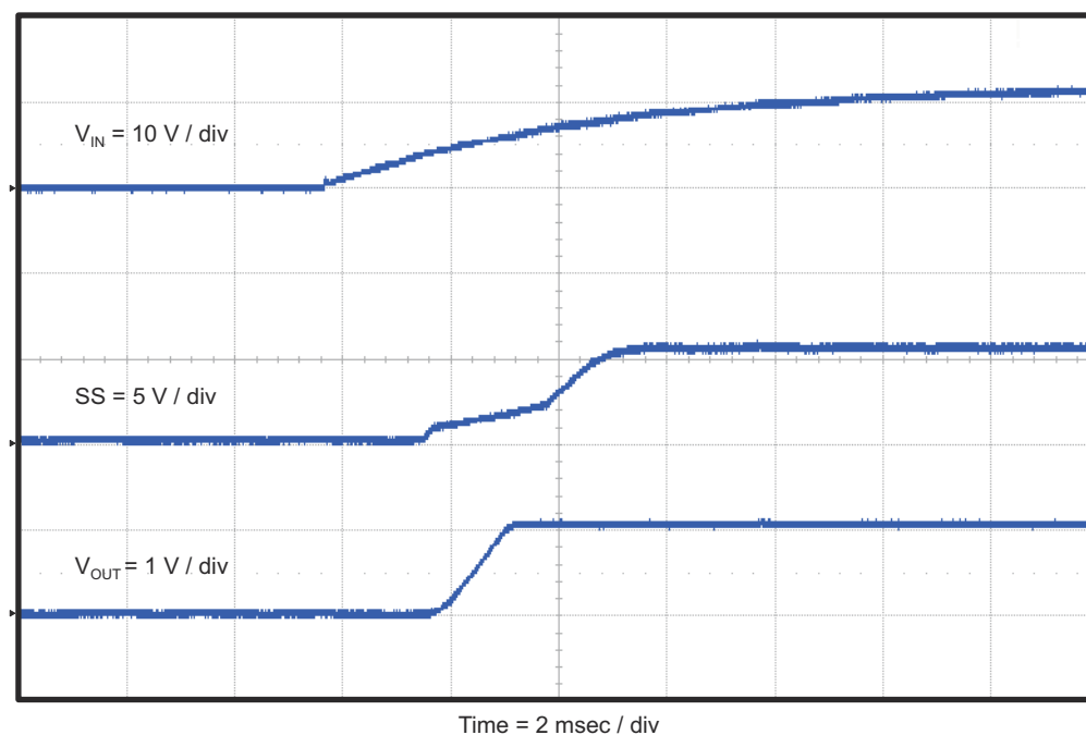
Figure 4-8. TPS54229EVM-056 Start-Up Relative to V_{IN} With SS
