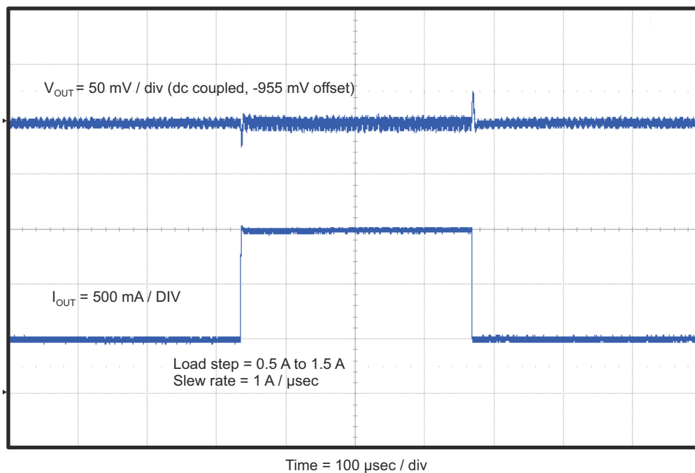
Figure 4-5. TPS54229EVM-056 Load Transient Response
