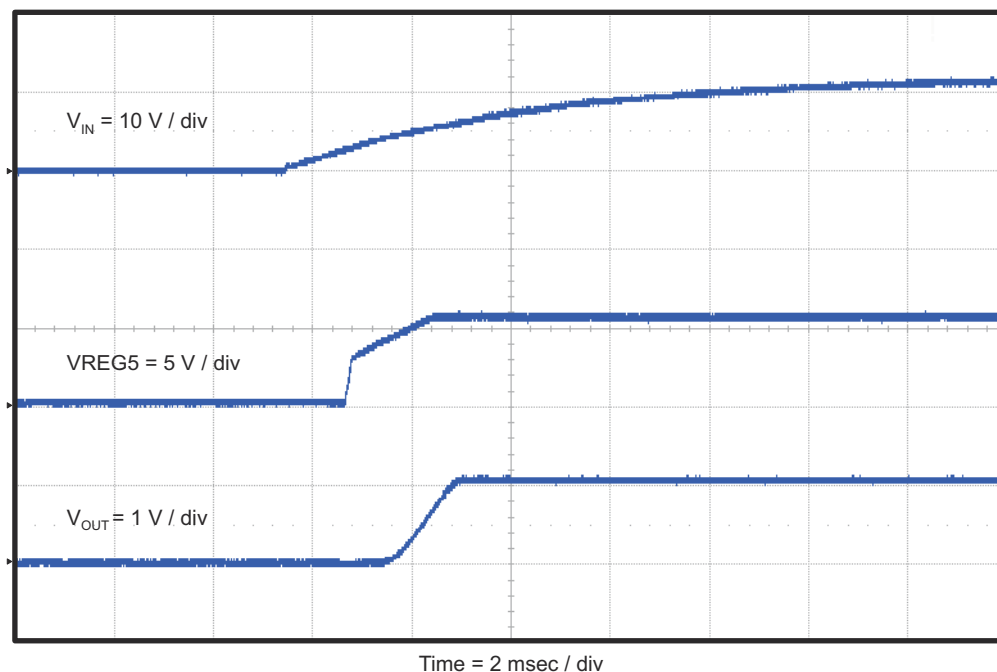
Figure 4-9. TPS54229EVM-056 Start-Up Relative to V_{IN} With VREG5
