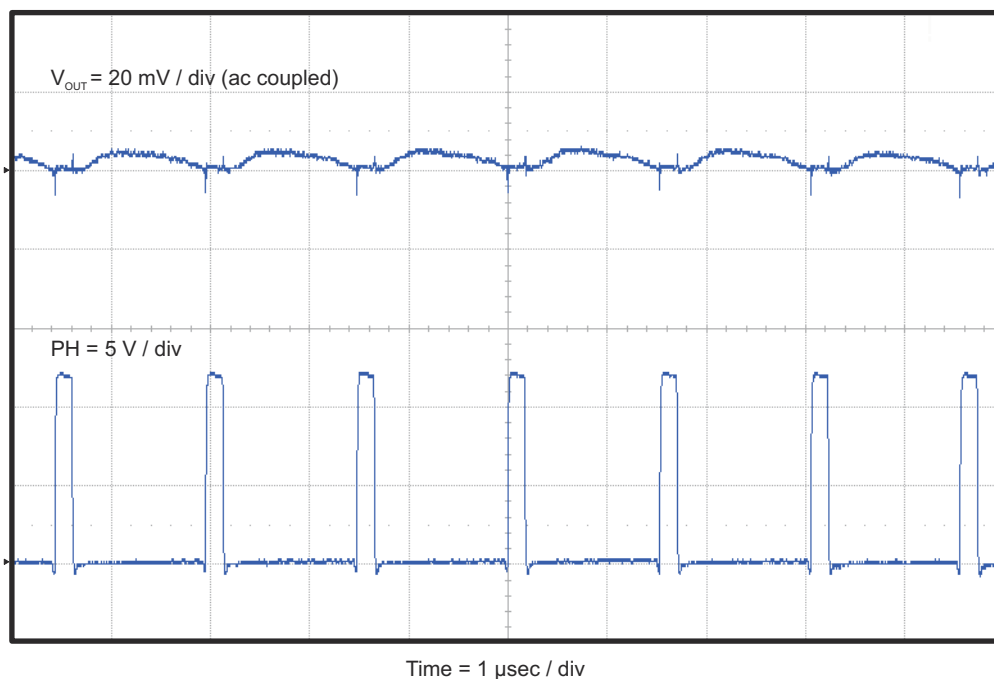
Figure 4-6. TPS54229EVM-056 Output Voltage Ripple
