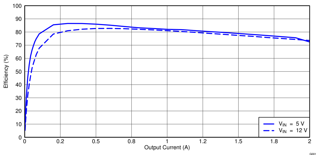
Figure 4-1. TPS54229EVM-056 Efficiency
