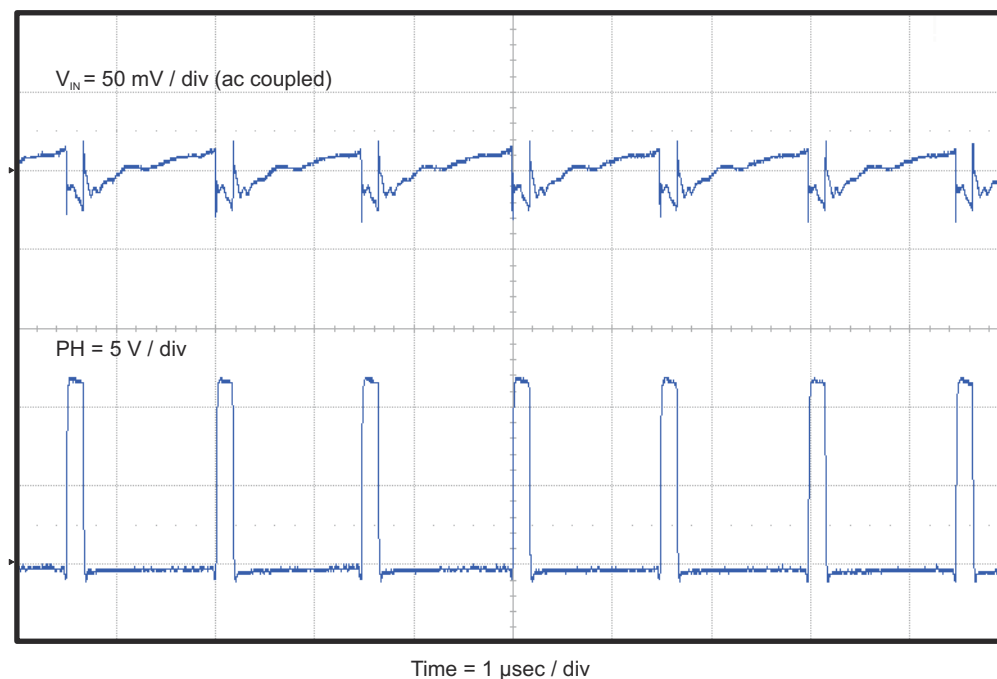
Figure 4-7. TPS54229EVM-056 Input Voltage Ripple
