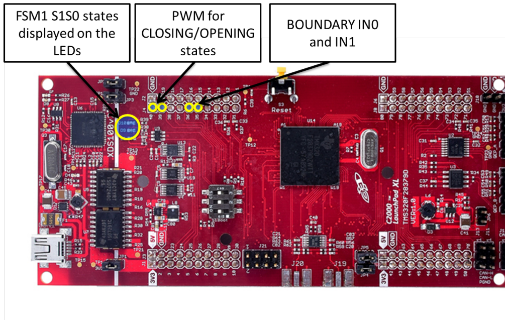
Figure 17. TSM320F28379D LaunchPad Connections
