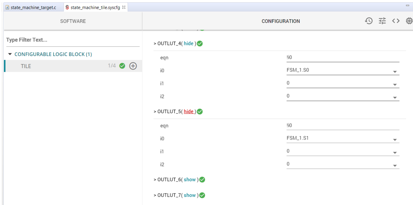
Figure 7. OUTLUT4 and OUTLUT5 Configurations
