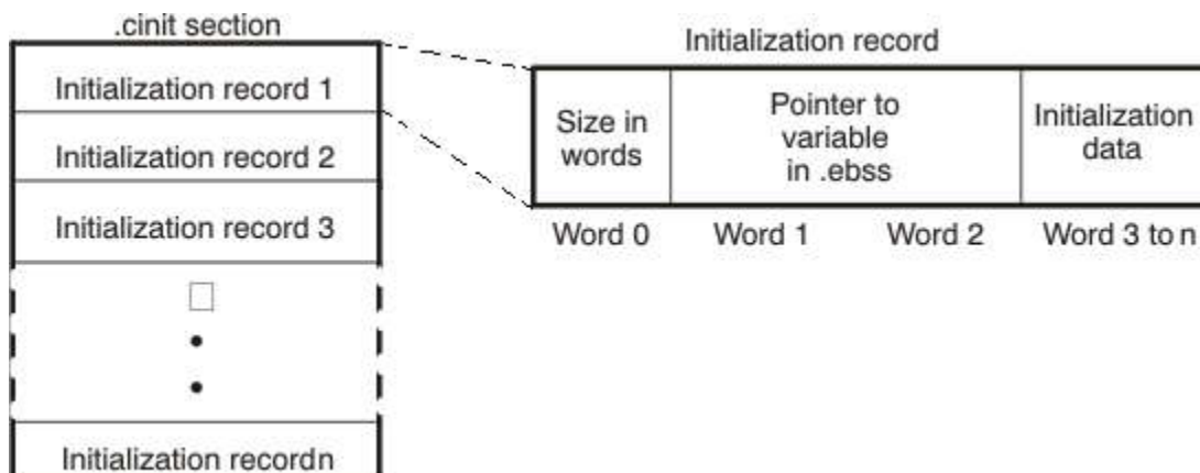
Figure 7-2. Format of Initialization Records in the .cinit Section (COFF)
