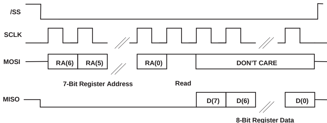
Figure 16. SPI Read
