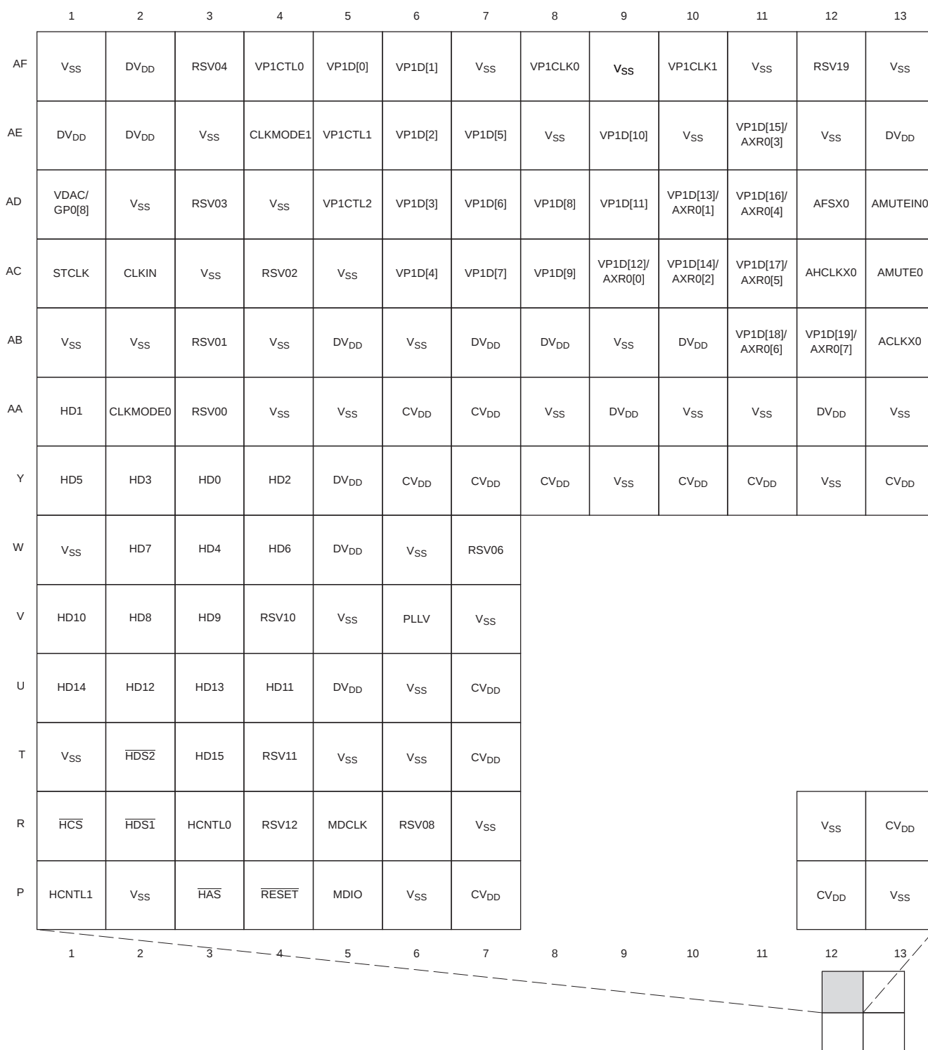
Figure 2-3. DM643 Pin Map [Quadrant A]
