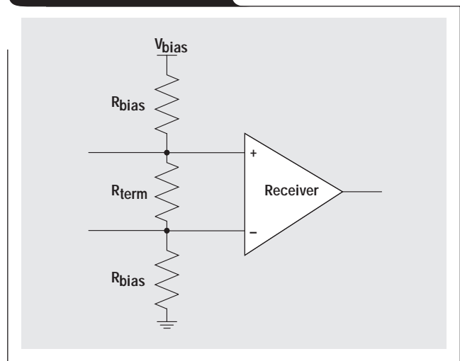
Figure 1. Input biasing
