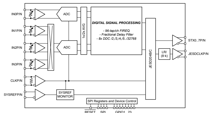
Block Diagram
