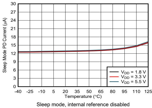
Figure 6-40. Power-Down Current vs Temperature
