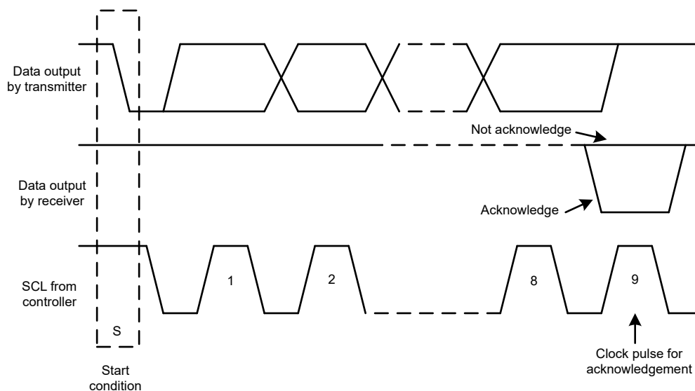
Figure 7-10. Acknowledge and Not Acknowledge on the I 2 C Bus
