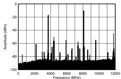
Figure 4-207. TX Single Tone Output Spectrum at 8.11 GHz
