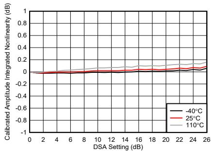
Figure 4-243. TX DSA Calibrated Amplitude Integrated Nonlinearity
