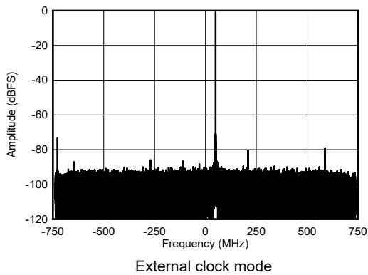
Figure 4-440. RX Single Tone Output FFT at 8.11GHz, -1dBFS
