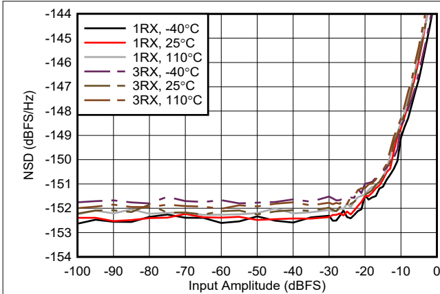
Figure 4-458. RX NSD vs Digital Amplitude at 9.6 GHz
