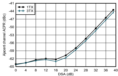
Figure 4-177. TX 20-MHz LTE ACPR vs DSA at 4.9 GHz
