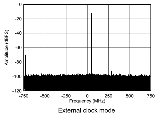
Figure 4-441. RX Single Tone Output FFT at 8.11GHz, -12dBFS
