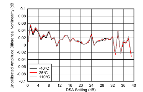
Figure 4-189. TX DSA Uncalibrated Amplitude Differential Nonlinearity at 8.1 GHz
