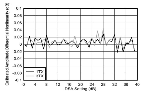
Figure 4-188. TX DSA Calibrated Amplitude Differential Nonlinearity at 8.1 GHz
