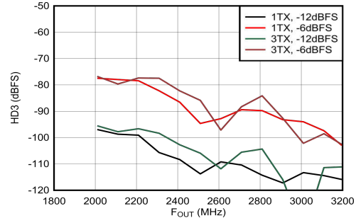
Matching at 2.6 GHz, f_{DAC} = 11.79648 GSPS, interleave mode, normalized to output power at harmonic frequency
