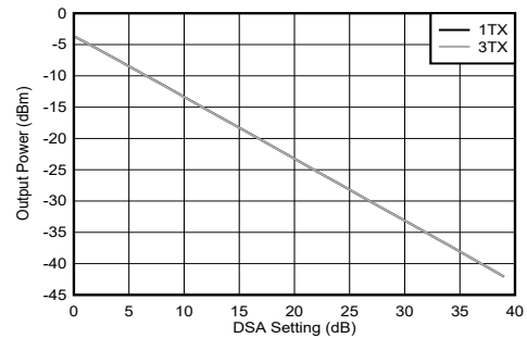
Figure 4-185. TX Output Power vs DSA Setting at 8.1 GHz
