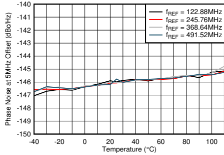
PLL enabled, f_{VCO} = 11796.48 MHz, measured at TX output
