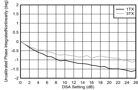
Figure 4-248. TX DSA Uncalibrated Phase Integrated Nonlinearity
