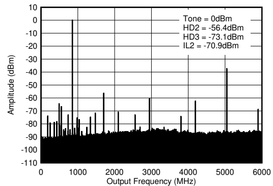
f_{DAC} = 5898.24 MSPS, interleave mode, 0.8 GHz matching, includes PCB and cable losses. IL_n = f_s/n \pm f_{OUT} .
