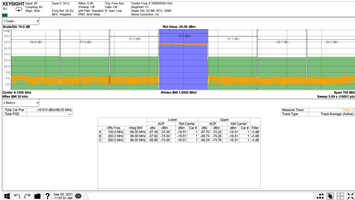
Figure 4-229. TX 100 MHz NR Output Spectrum at 8.1 GHz
