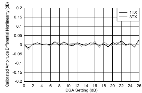
Figure 4-237. TX DSA Calibrated Amplitude Differential Nonlinearity
