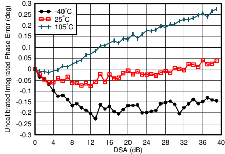
f_{\text{DAC}} = 8847.36 MSPS, straight mode, matching at 2.6 GHz, channel with the medium variation over DSA setting at 25°C Integrated Phase Error = Phase(DSA Setting) – Phase(DSA Setting = 0)
