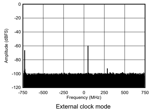
Figure 4-443. RX Single Tone Output FFT at 8.11GHz, -60dBFS
