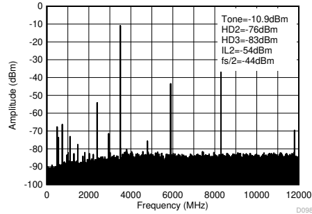
Figure 4-148. TX Single Tone (-12 dBFS) Output Spectrum at 3.5 GHz (0- f_{\text{DAC}} )
