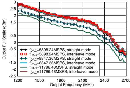
Figure 4-44. TX Output Fullscale vs Output Frequency
