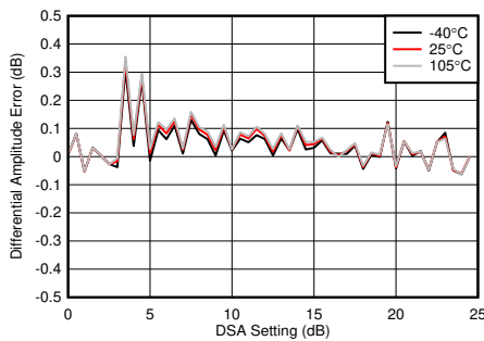
Figure 4-366. RX In-Band Gain Flatness, f_{IN} = 3600\text{ MHz}
