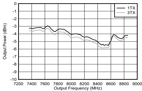
Figure 4-184. TX Output Power vs Frequency at 8.1 GHz
