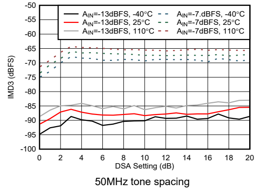
Figure 4-429. RX IMD3 vs DSA Setting at 8.1GHz
