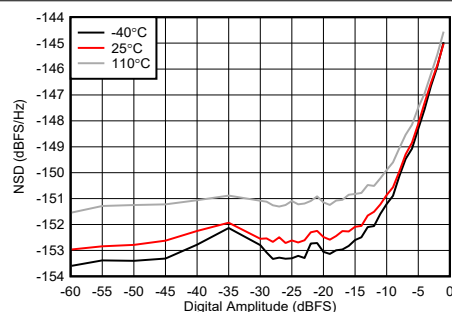
Figure 4-260. TX NSD vs Digital Amplitude at 9.61 GHz
