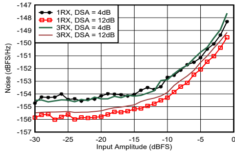
Figure 4-299. RX Noise Spectral Density vs Input Amplitude and Channel at 0.8 GHz
