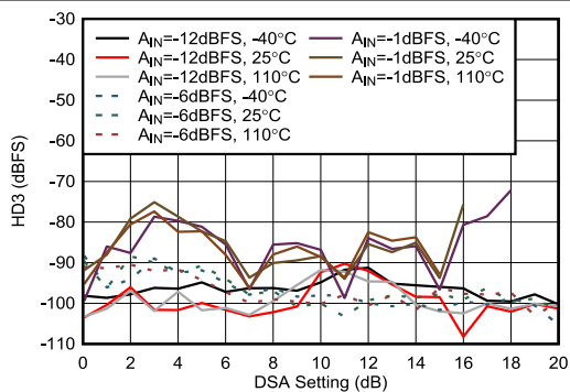
Figure 4-438. RX HD3 vs DSA Setting at 8.1GHz
