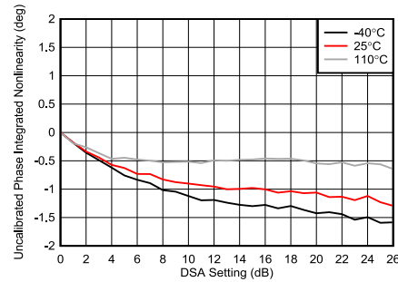
Figure 4-250. TX DSA Uncalibrated Phase Integrated Nonlinearity
