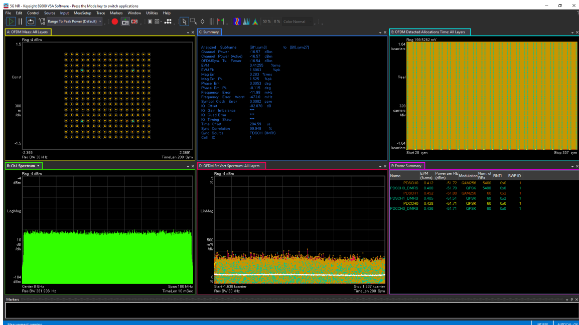
Figure 4-230. TX 100 MHz NR EVM at 8.1 GHz
