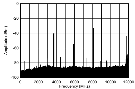
50 MHz tone spacing, -30 dBFS each tone
