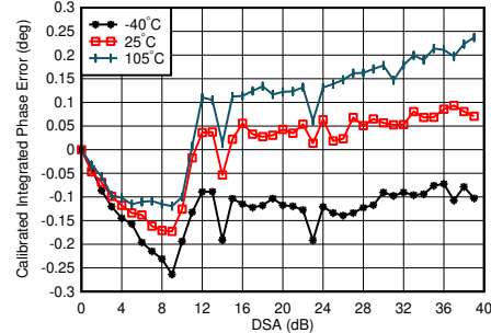
f_{\text{DAC}} = 8847.36 MSPS, straight mode, matching at 2.6 GHz, channel with the median variation over DSA setting at 25°C Integrated Phase Error = Phase(DSA Setting) – Phase(DSA Setting = 0)
