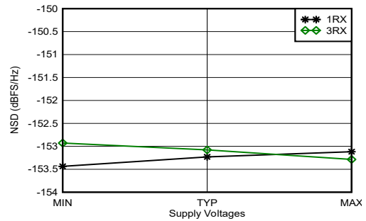
Figure 4-365. RX Noise Spectral Density vs Supply and Channel at 2.6 GHz
