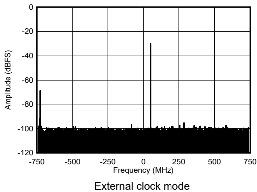
Figure 4-442. RX Single Tone Output FFT at 8.11GHz, -30dBFS
