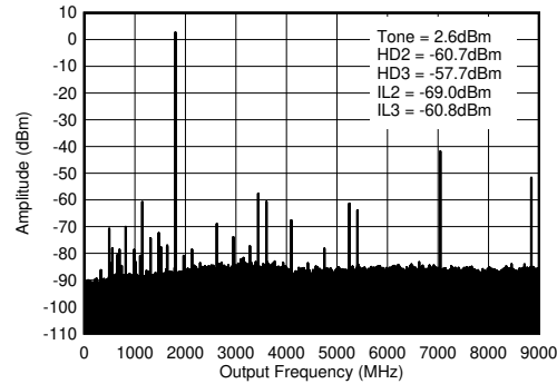
Figure 4-75. TX Single Tone (-12 dBFS) Output Spectrum at 1.8 GHz ( 0-f_{DAC} )
