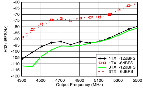
Matching at 4.9 GHz, f_{DAC} = 11.79648 GSPS, interleave mode, normalized to output power at harmonic frequency
