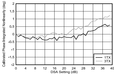
Figure 4-200. TX DSA Calibrated Phase Integrated Nonlinearity at 8.11 GHz
