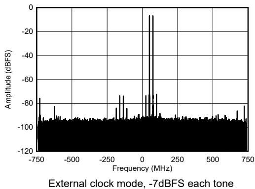
Figure 4-444. RX Dual Tone Output FFT at 8.11GHz
