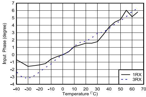
Figure 4-287. RX Input Phase vs Temperature and DSA at f_{OUT} = 0.8\text{ GHz}
