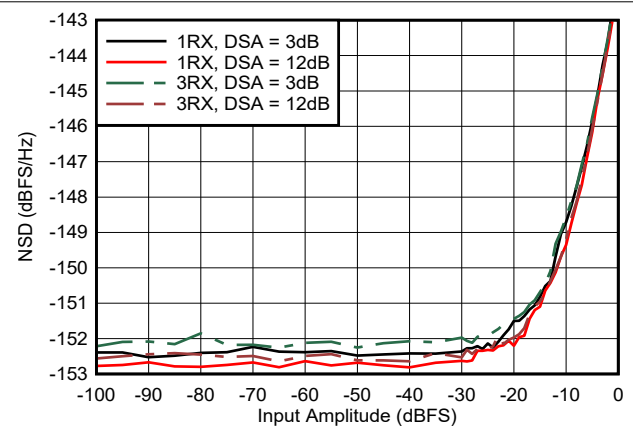
Figure 4-459. RX NSD vs Digital Amplitude at 9.6 GHz
