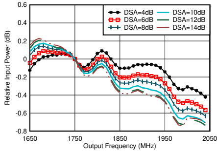
Figure 4-316. RX In-Band Gain Flatness, f_{IN} = 1750\text{ MHz}
