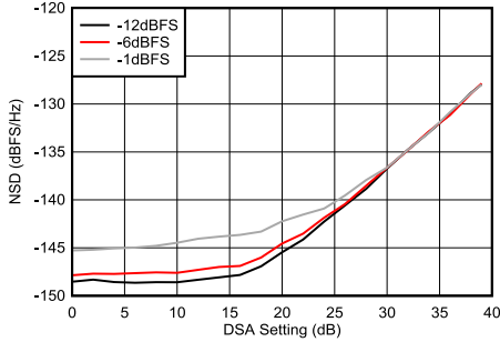
Figure 4-261. TX NSD vs DSA Setting at 9.61 GHz
