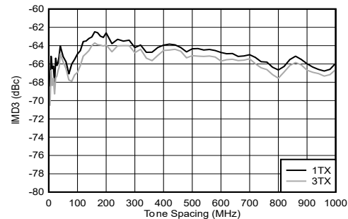
Figure 4-256. TX IMD3 vs Tone Spacing at 9.61 GHz
