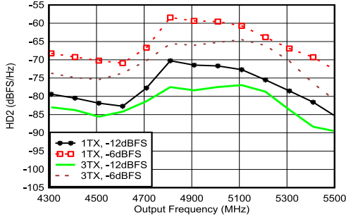
Matching at 4.9 GHz, f_{DAC} = 11.79648 GSPS, interleave mode, normalized to output power at harmonic frequency
