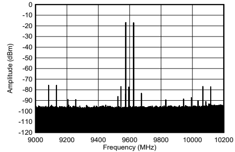
Figure 4-274. TX 2-Tone Spectrum at 9.61 GHz and -13 dBFS (1.2 GHz BW)
