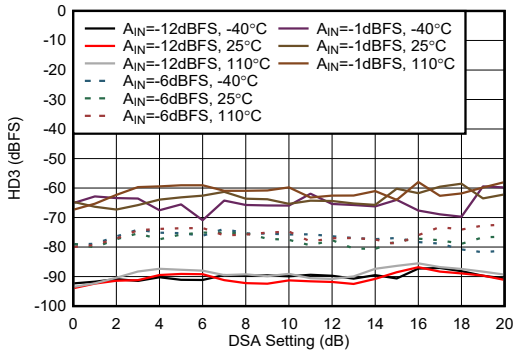
Figure 4-464. RX HD3 vs DSA Setting at 9.6 GHz
