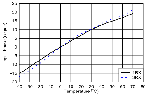
Figure 4-318. RX Input Phase vs Temperature and DSA at f_{IN} = 1.75\text{ GHz}
