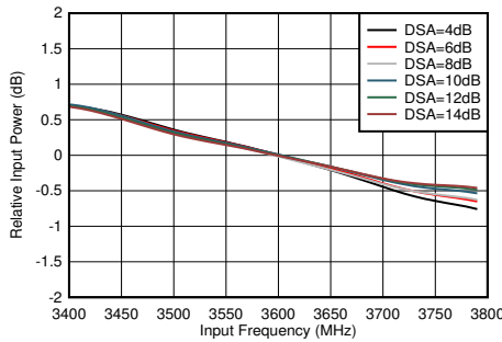
Figure 4-366. RX In-Band Gain Flatness, f_{IN} = 3600\text{ MHz}
