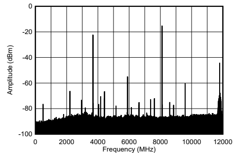
Figure 4-205. TX Single Tone Output Spectrum at 8.11 GHz
