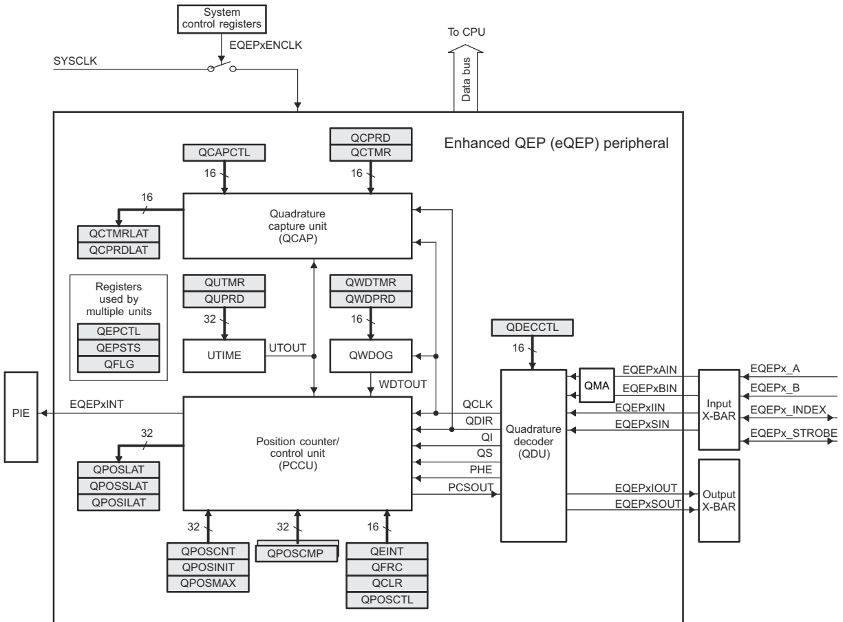
Figure 6-5. eQEP Block Diagram
