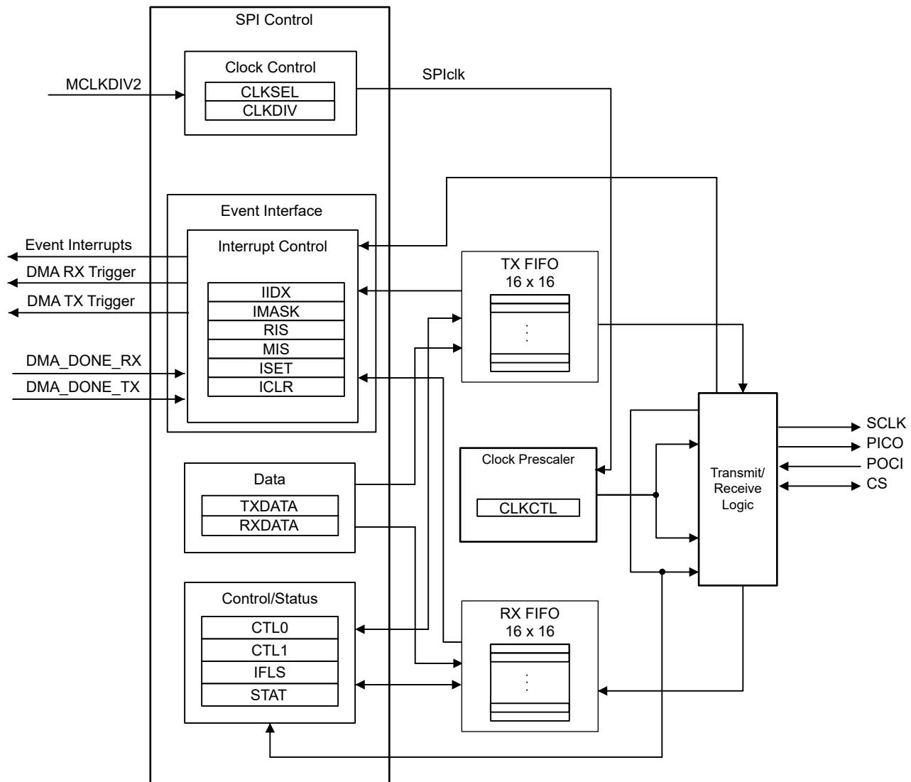
Figure 7-6. SPI Functional Block Diagram
