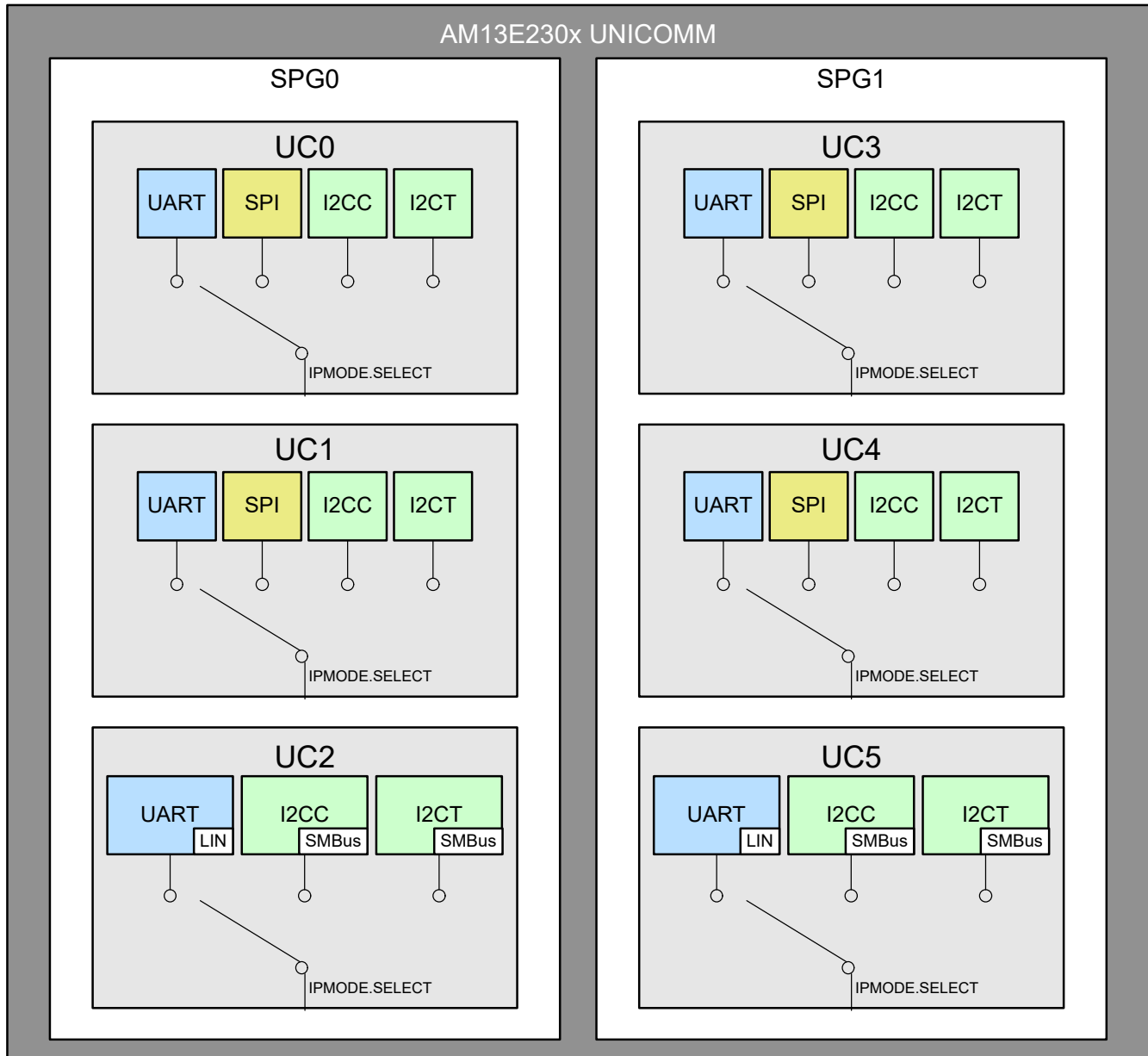
Figure 7-2. Unicomm Block Diagram
