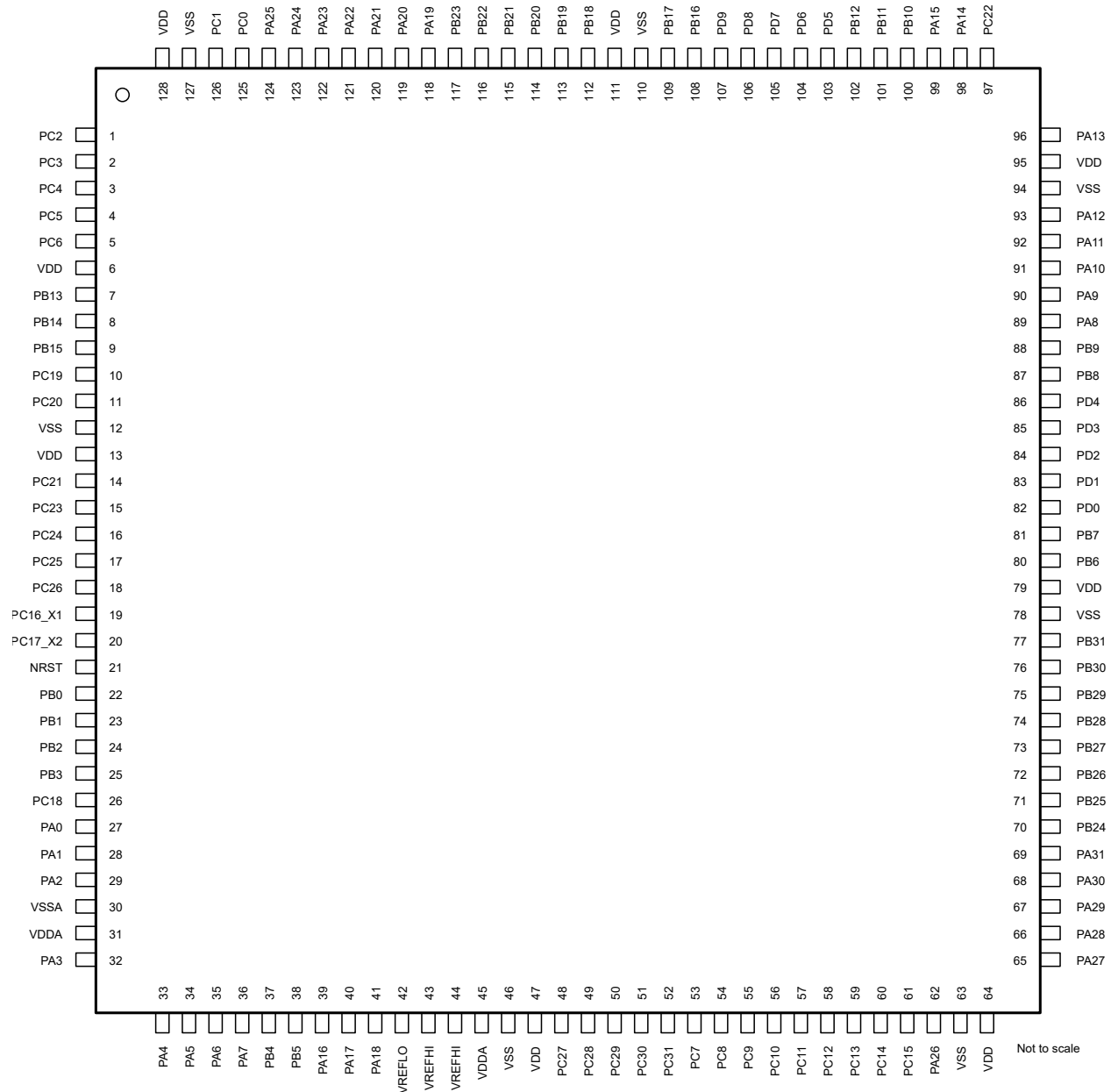
Figure 5-1. LQFP128 (PDT) Package
