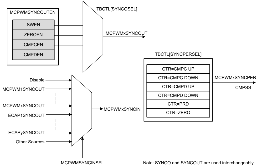
Figure 6-2. Synchronization Chain Architecture
