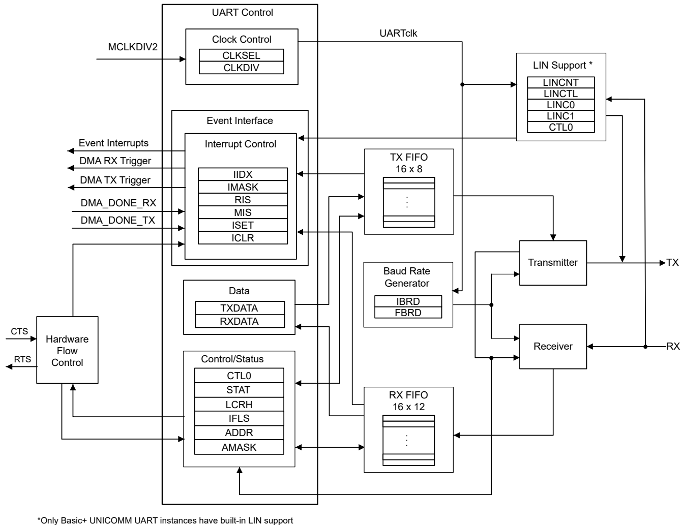
Figure 7-3. UART Functional Block Diagram
