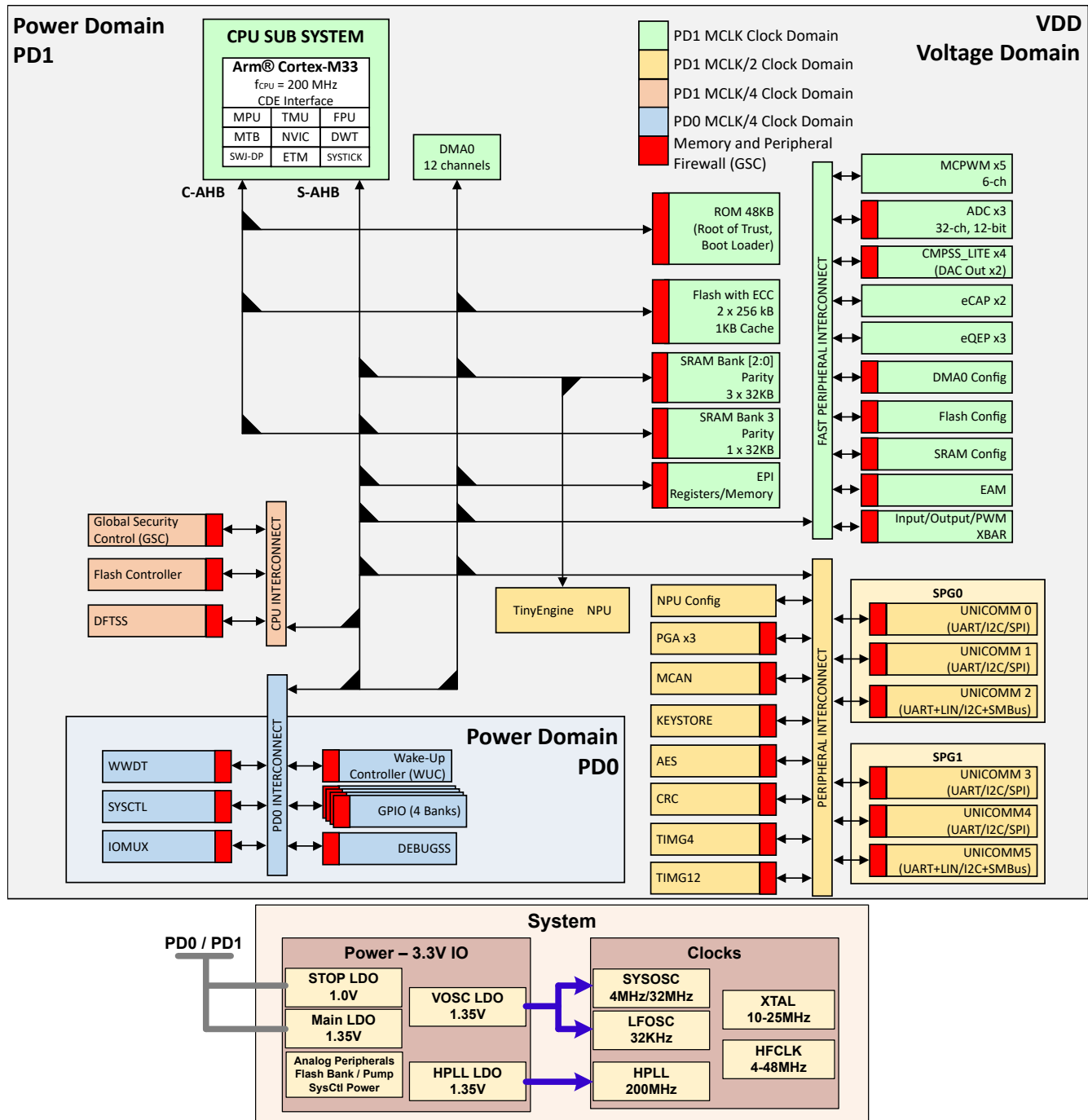
Figure 7-1. AM13E230x Functional Block Diagram
