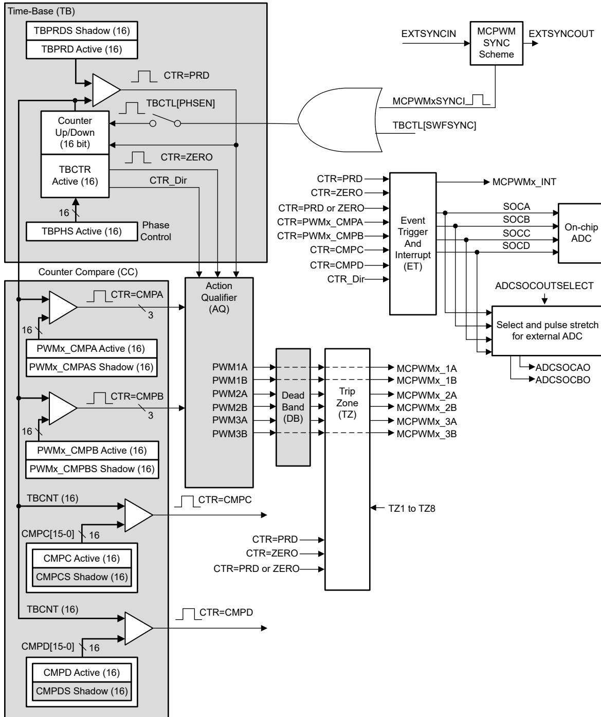
Figure 6-1. MCPWM Submodules and Critical Internal Signal Interconnects
