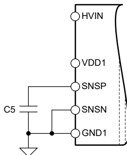
Figure 8-2. Input Filter
