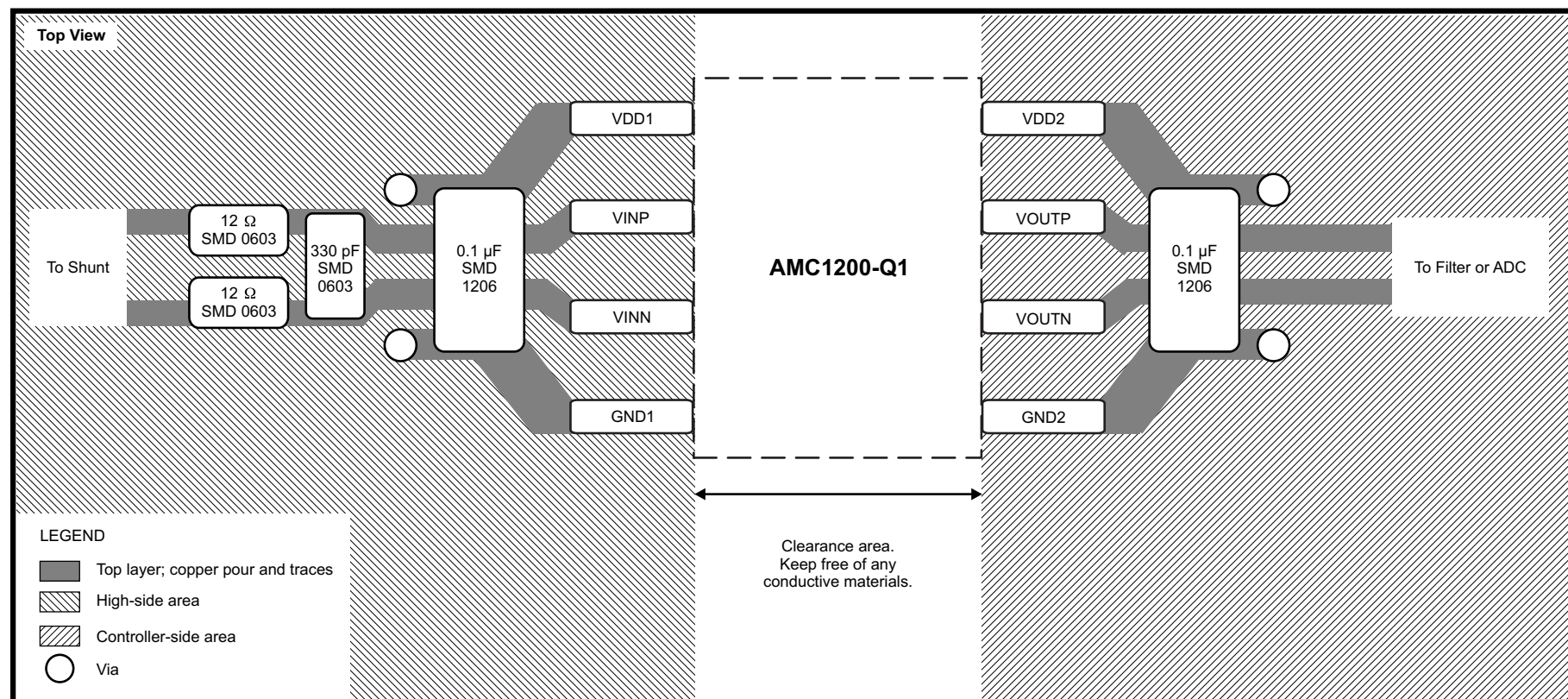
Figure 37. Layout Recommendation
