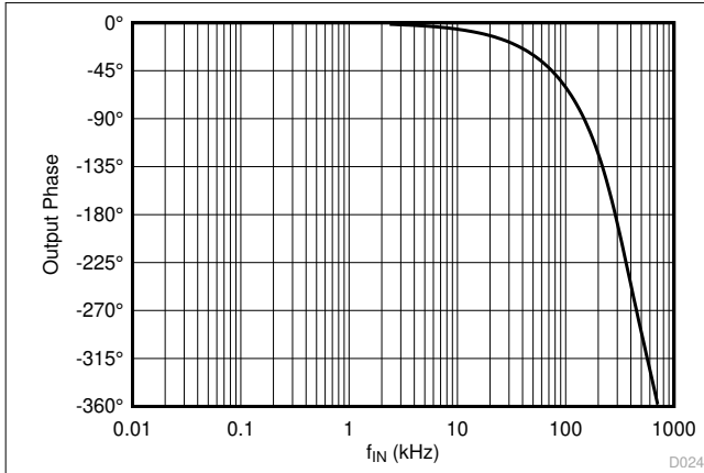
Figure 6-17. Output Phase vs Input Frequency
