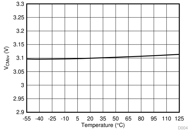
Figure 6-6. Common-Mode Overvoltage Detection Level vs Temperature
